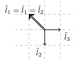
FIGURE 9. The fan for L_{\mathcal{O}_E(E)}b^*\mathcal{O}(2), \mathcal{O}_E(E)[1], b^*\mathcal{O}(3), b^*\mathcal{O}(4) .
