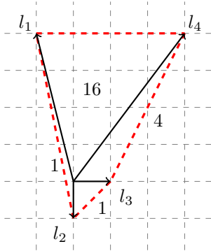
FIGURE 5. The fan for b^*\mathcal{T}, \mathcal{R}', b^*\mathcal{O}(2), b^*\mathcal{O}(4) .
