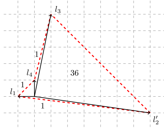
FIGURE 2. The fan associated to \mathcal{O}, \mathcal{O}(2P+Q), \mathcal{R}, \mathcal{O}(3P+Q) on \mathbb{F}_3 .
