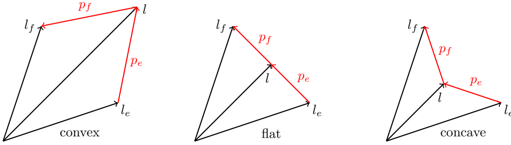
FIGURE 10. Convex, flat, and concave configurations of l_e, l, l_f for a < 0 .
