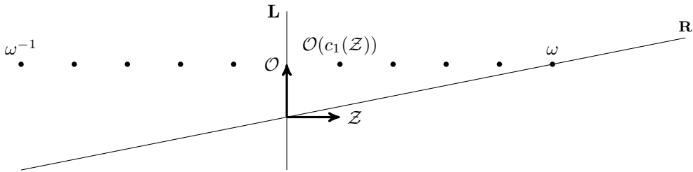
FIGURE 7. The configuration of \mathbf{L} and \mathbf{R} in L for \delta_{\mathcal{Z}} = 2 .
