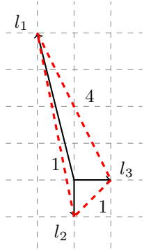
FIGURE 3. The fan associated to \mathcal{T}, \mathcal{O}(2), \mathcal{O}(4) on \mathbb{P}^2 .
