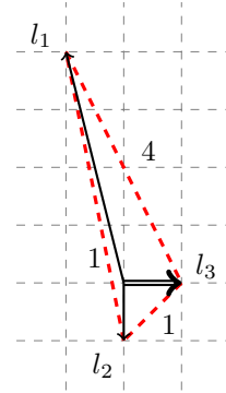
FIGURE 4. The fan associated to \mathcal{O}_E(E), b^*\mathcal{T}, b^*\mathcal{O}(2), b^*\mathcal{O}(4) on X .
