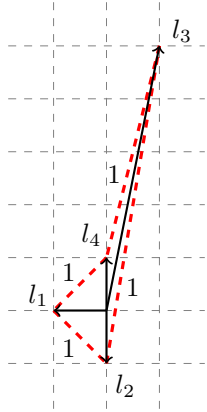
FIGURE 1. The fan associated to \mathcal{O}, \mathcal{O}(P), \mathcal{O}(2P+Q), \mathcal{O}(3P+Q) on \mathbb{F}_3 .
