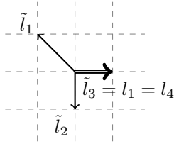
FIGURE 8. The fan for \mathcal{O}_E(E), b^*\mathcal{O}(2), b^*\mathcal{O}(3), b^*\mathcal{O}(4) .
