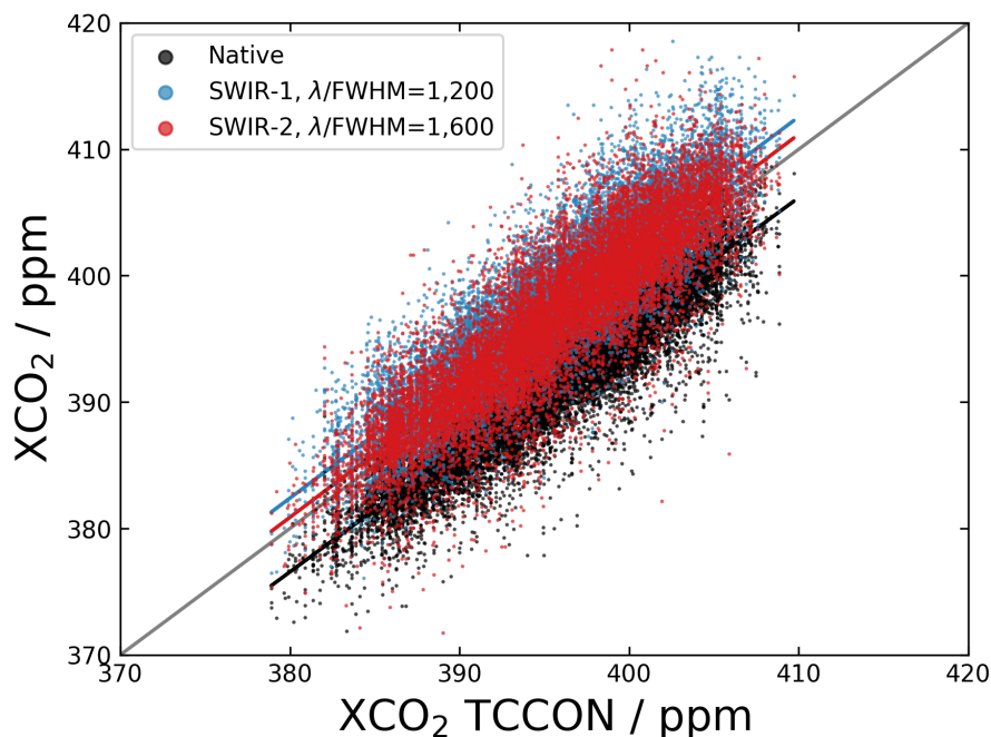
Figure 4. Correlation between XCO_2 retrieved from GOSAT with the TCCON network. Black: native GOSAT retrieval; Blue: SWIR-1 retrieval at 1,200 resolving power; Red: SWIR-2 retrieval at 1,600 resolving power. The grey line indicates a 1:1 correlation line; the colored lines show linear fits to the respective dataset. Standard deviations around TCCON amount to 2.43 ppm (native, compare e.g. Guerlet et al. (2013b)), 3.00 ppm (SWIR-1) and 3.28 ppm (SWIR-2).
