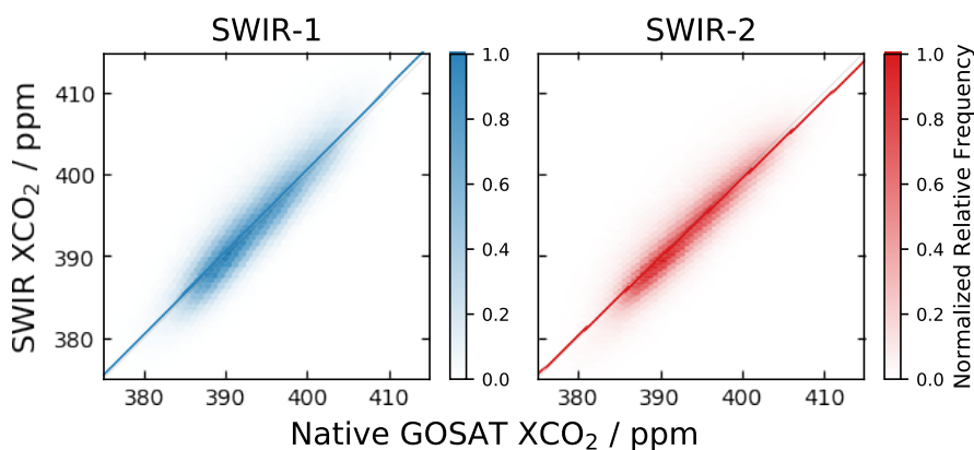
Figure 7. Retrieved SWIR-1 (left) and SWIR-2 (right) XCO 2 plotted versus the corresponding native GOSAT retrievals. The colored lines indicate linear fits to the data, the grey line marks the 1:1 correlation. Scatter amounts to 2.85 ppm and to 2.69 ppm in SWIR-1 and SWIR-2, respectively. Color shading encodes relative occurrence of data points.
