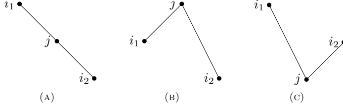
FIGURE 3. The three possible ways the i_1, j, i_2 piece of \tilde{\sigma} = \sigma \circ (i_1 \ j) can look like, when (i_1, i_2) is a \sigma -drop: i_1 < j < i_2 (A), j > i_1, i_2 (B), and j < i_1, i_2 (C). The \sigma -drop (i_1, i_2) is drop-admissible in case (A), and jump-admissible in (B) and (C).
