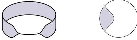
Figure 1.1: A pair of degenerate annuli, one (from [Hen14]) depicted in three space, and another embedded in the complex plane.
