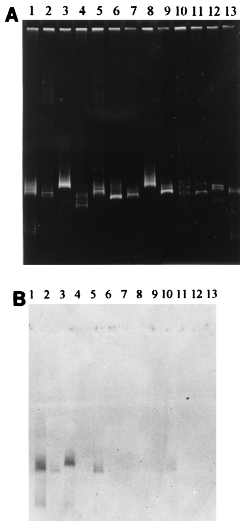
FIG. 3. (A) DGGE separation patterns for PCR-amplified 16S rDNA segments derived from pure cultures of ferrous iron-oxidizing, nitrate-reducing bacteria and cultures from mixotrophic MPN dilution series inoculated with sediment samples collected in Bremen in June 1996. Three parallel MPN culture series (series 1 to 3) were analyzed. Lane 1, strain BrG1; lane 2, dilution 1 \cdot 10^3 ; lane 3, dilution 1 \cdot 10^4 ; lane 4, dilution 1 \cdot 10^5 ; lane 5, dilution 2 \cdot 10^3 ; lane 6, dilution 2 \cdot 10^4 ; lane 7, dilution 2 \cdot 10^5 ; lane 8, dilution 2 \cdot 10^6 ; lane 9, dilution 2 \cdot 10^7 ; lane 10, dilution 3 \cdot 10^3 ; lane 11, dilution 3 \cdot 10^4 ; lane 12, dilution 3 \cdot 10^5 ; lane 13, strain BrG3. (B) DGGE gel in panel A after blotting onto a nylon membrane and hybridization with the oligonucleotide probe specific for strain BrG1.
