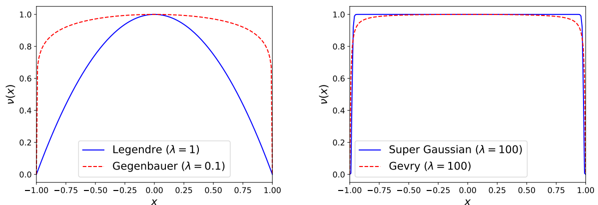
(a) Legendre viscosity ( \lambda = 1 ) and Gegenbauer viscosity for \lambda = 0.1 (b) Super Gaussian viscosity and Gevrey viscosity for \lambda = 100
