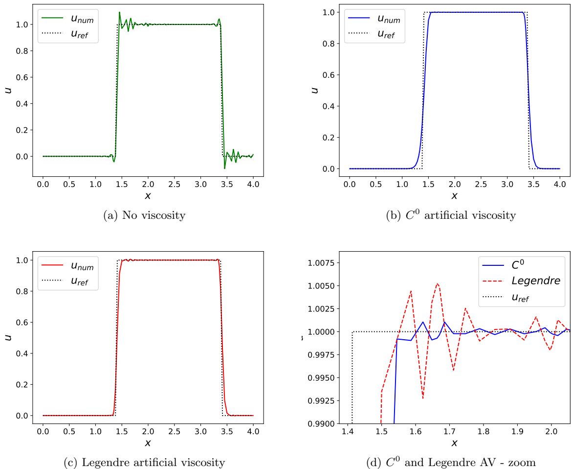
Figure 4: Numerical solutions and viscosities for the linear advection equation using 12 elements and polynomials of degree 10 or less.
