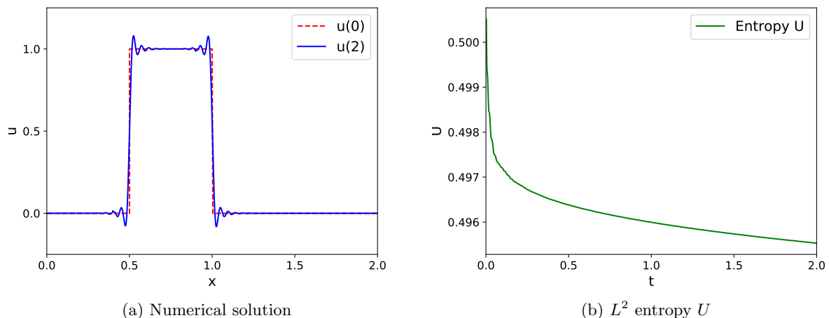
Figure 1: Numerical solution and its entropy for linear advection using N = 20 elements with polynomials of degree \leq p = 9 , 1 000 timesteps of the SSPRK(3,3) method, and a full upwind numerical flux.
