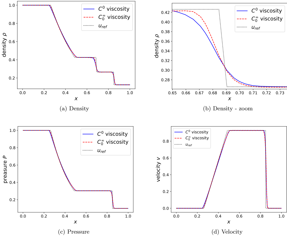
Figure 6: Numerical solutions for Sod's shock tube.
