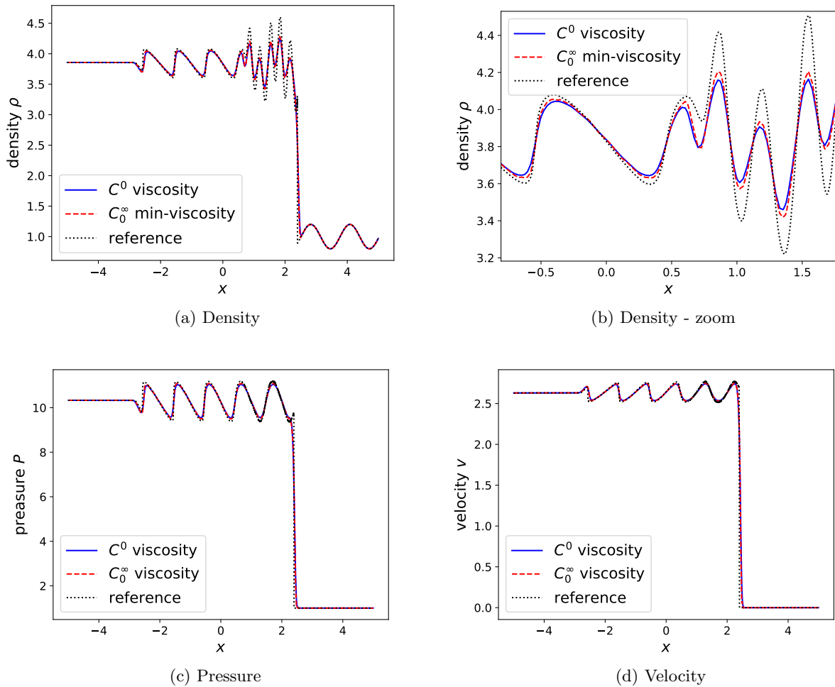
Figure 7: Numerical solutions for Shu and Osher's shock tube.
