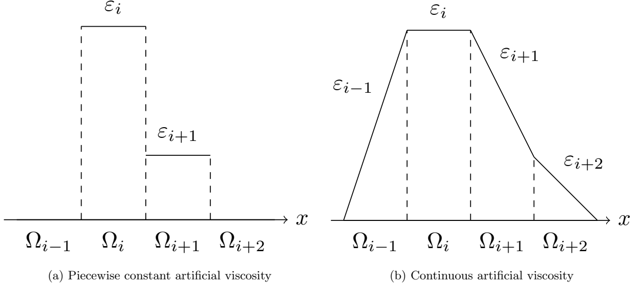
Figure 3: A piecewise constant viscosity and the corresponding continuous viscosity constructed by the algorithm of Klöckner et al..
