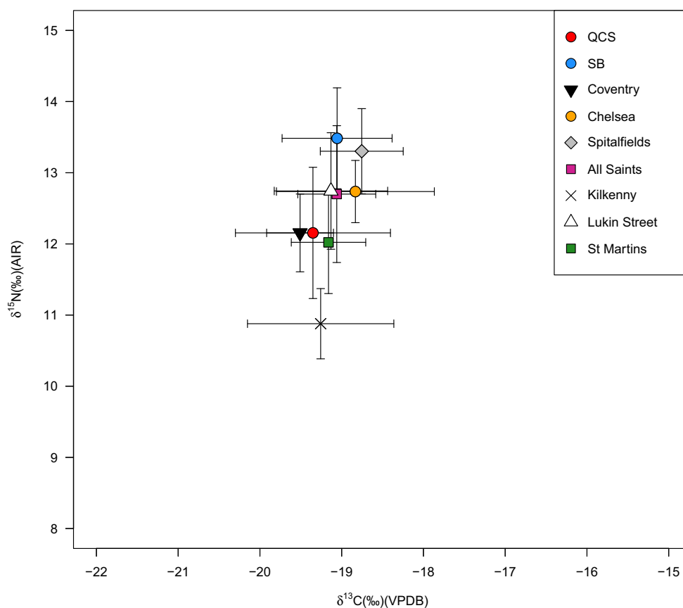
Fig. 7 Adult \delta^{13}\text{C}_{\text{coll}} and \delta^{15}\text{N}_{\text{coll}} mean values and standard deviations for the post-medieval sites of Chelsea ( n = 28 ), Lukin Street, London ( n = 64 ), Christ Church Spitalfields, London ( n = 88 ), All Saints, York ( n = 10 ), Coventry ( n = 11 ), St Martin's, Birmingham ( n = 18 ) and Kilkenny Workhouse, Ireland ( n = 14 ) (Trickett 2006; Beaumont et al. 2013a; Nitsch et al. 2010; Müldner and Richards 2007a; Richards 2006). QCS is marked in red and SB in blue. Adults are defined as individuals being 18 years of age or above
