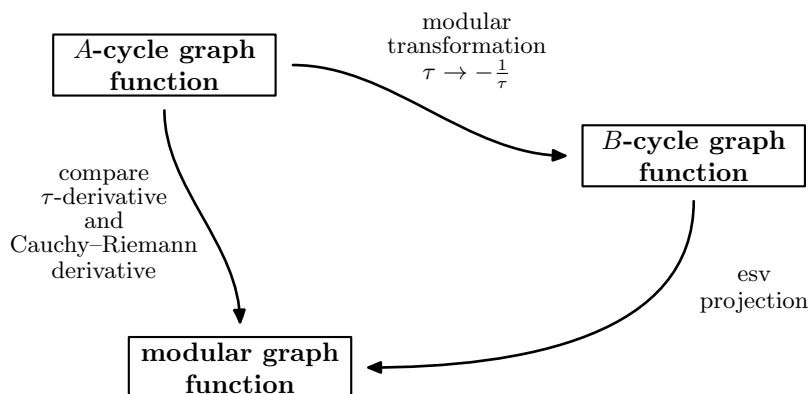
Figure 3. Two paths for the calculation of modular graph functions.
