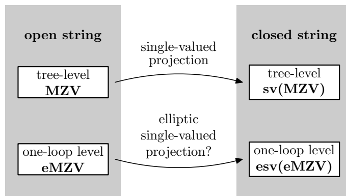
Figure 1. Context of a tentative generalization “esv” of the single-valued projection to genus one.
