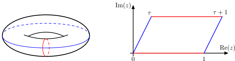
Figure 2. Parametrization of a torus as a lattice \mathbb{C}/(\mathbb{Z}+\tau\mathbb{Z}) with modular parameter \tau in the upper half plane and complex coordinate z \cong z+1 \cong z+\tau . The homology cycle drawn in red is mapped to the unit interval (0, 1) and referred to as the A -cycle. Accordingly, the second homology cycle mapped to the path from 0 to \tau is known as the B -cycle.
