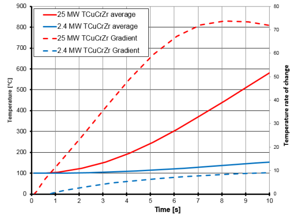
Fig. 8 Example of thermal gradient for two extreme NBI beam dump power densities ( \text{MW}/\text{m}^2 )
