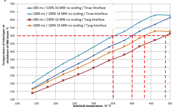
Fig. 7 Relation between TC temperature limit and NBI shutdown temperature of the interlayer depending on NBI power density ( \text{MW}/\text{m}^2 ) and total reaction time.
