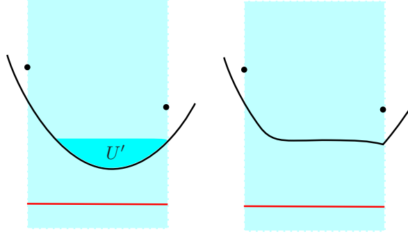
FIGURE 5. Isotopy for a strand of Type II.
