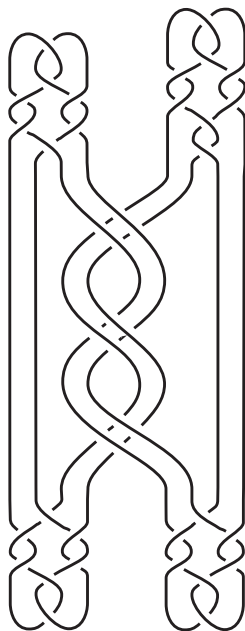
FIGURE 13. A minimal crossing diagram D of a prime knot K such that w(D) = \beta(K) = 4 .
