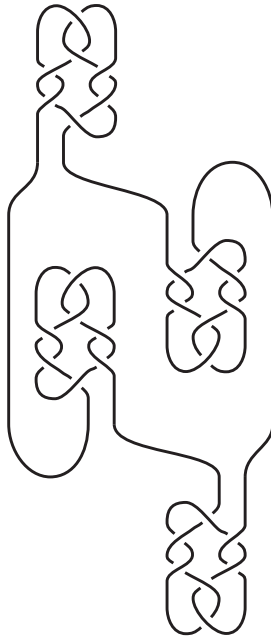
FIGURE 11. A minimal crossing diagram D of a composite knot K such that \omega(D) = 6 and \beta(K) = 5 . Additionally, b_{||}(D) = 7 .
