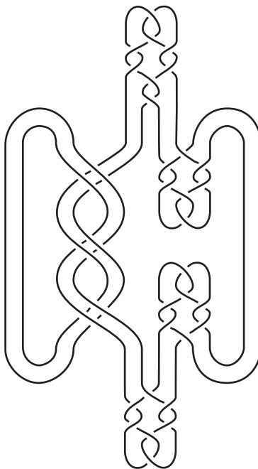
FIGURE 12. A minimal crossing diagram D of a prime knot K such that \omega(D) = 6 and \beta(K) = 4 .
