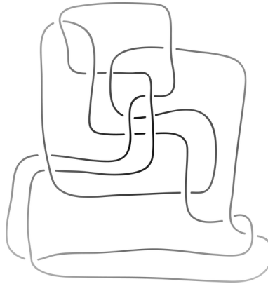
FIGURE 10. The Thistlethwaite unknot, whose Wirtinger number is 3.
