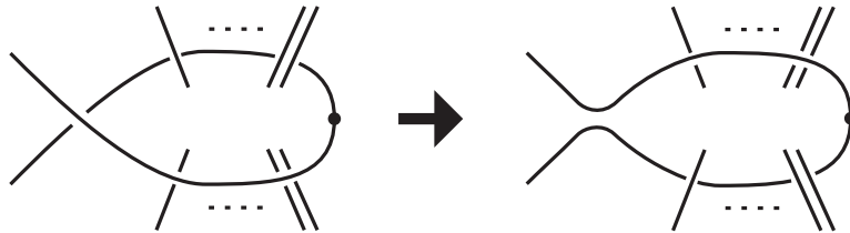
FIGURE 3. Reducing the crossing number.
