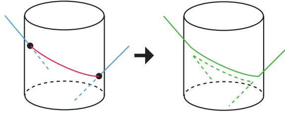
FIGURE 9. Surgering \gamma along \hat{\alpha}
