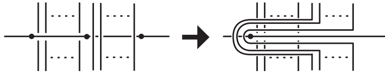
FIGURE 2. Reducing the overpass bridge number.
