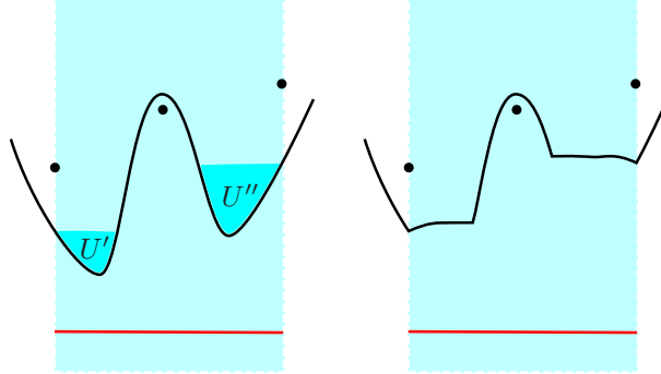
FIGURE 7. Isotopy for a strand of Type IV.
