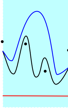
FIGURE 4. Isotopy decreasing the number of critical points for \hat{s}_i , if it contains more than three critical points of h|_\gamma . The red line is the projection, s_i , and the black dots represent the lifts of strands over which s_i passes.
