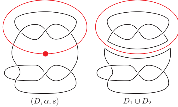
FIGURE 8. An example of the triple (D, \alpha, s) inducing a pair of diagrams D_1 and D_2 . The red dot is s and specifies the arc along which the diagram is surgered.
