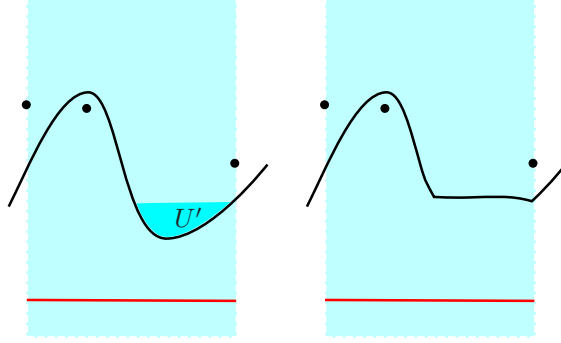
FIGURE 6. Isotopy for a strand of Type III.
