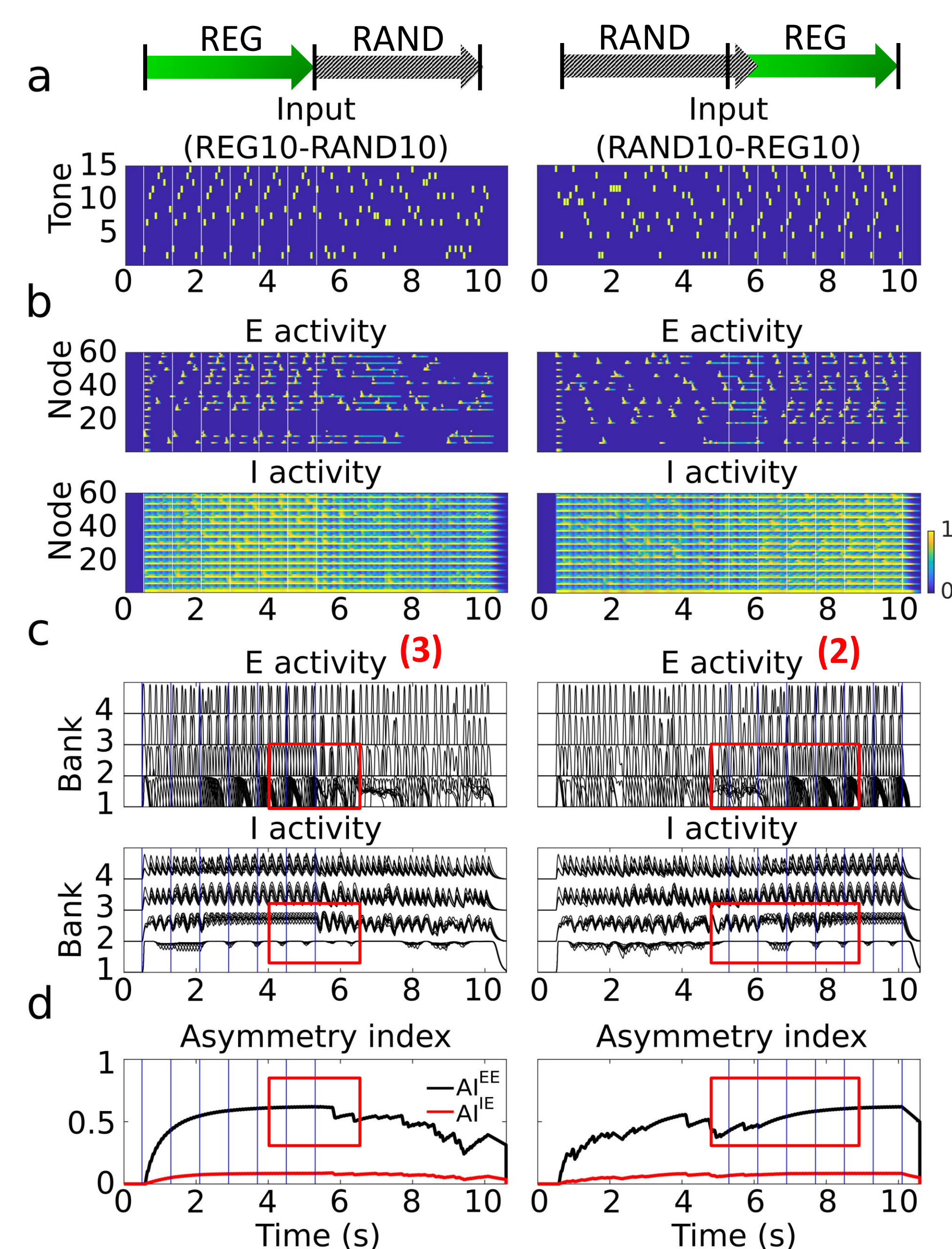
Fig. 1. Simulation examples of REG10-RAND10 and RAND10-REG10. (a) The inputs. (b) The E/I activity. (c) The E/I activity shown separately in four resonance frequencies. Here we can see that the E/I activity (regularity representation) decreases quickly at the transition from REG to RAND (3), and increase gradually at the transition from RAND to REG (2). (d) The asymmetry index (AI) of W^{EE} and W^{IE} takes a few repetitions to reach its plateau.
