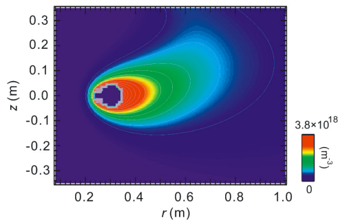
Fig. 3: A plasma confined in RT-1, a laboratory "artificial magnetosphere" generated by a superconducting (SC) levitated dipole coil (lhs), and an example for a self-organized peaked density profile of a plasma in RT-1 (rhs) 25,27
