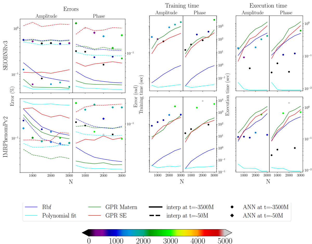
Figure 5. The seven-dimensional interpolation results. Top:SEOBNRv3, bottom:IMRPhenomPv2. The x -axes show the number of training points N and the y -axes shows the errors, training, and execution time as shown on the plot. Left: errors of the amplitude ( A(t) ) and phase ( \phi(t) ) respectively, middle: training time in unit seconds, and right: execution time in unit seconds. The solid lines show the results at t = -3500M and the dashed lines for t = -50M . Different colors represent different interpolation methods as shown in the shared legend. The colored circles correspond to the results of ANN at t = -3500M and the colored diamonds for t = -50M . Different colors represent a different number of neurons on a double layer ANN as shown in the corresponding color bar.
