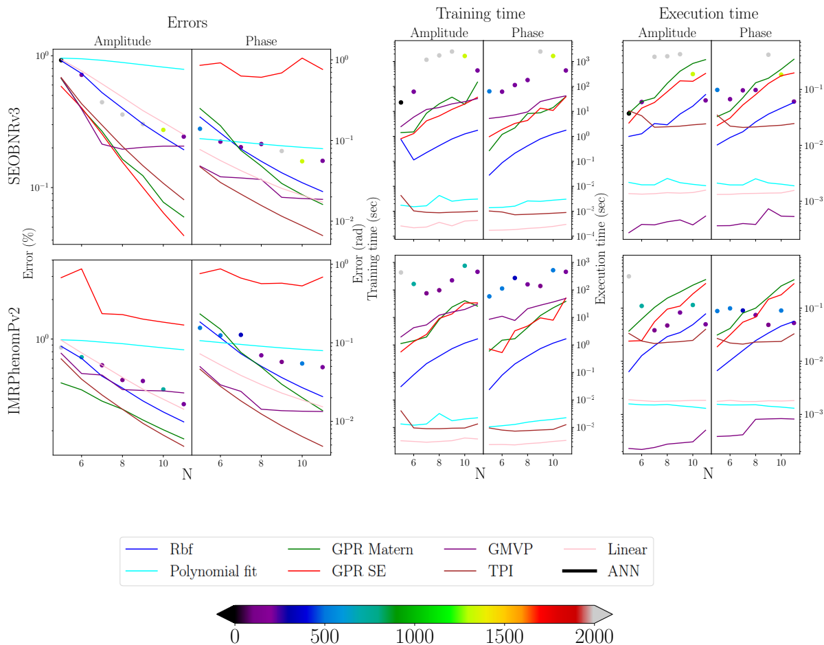
Figure 3. The three-dimensional interpolation results at t=-3500M . Top: SEOBNRv3, bottom: IMRPhenomPv2. The x -axes show the number of training points in each dimension, N , and the y -axes show the errors, training, and indicated execution time as on the labels of the panels. Left: errors of the amplitude and phase respectively, middle: training time in (seconds), and right: execution time (seconds). Different colors represent different interpolation methods as shown in the shared legend. The colored circles show ANN results, where different colors represent the number of neurons per layer in a double layer ANN as shown in the corresponding color bar.
