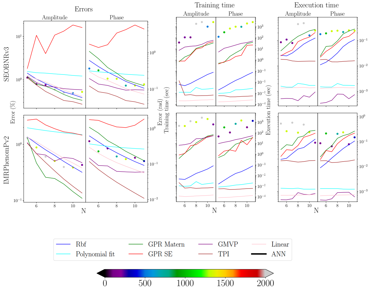
Figure 4. The three-dimensional interpolation results at t=-50M . Top:SEOBNRv3, bottom:IMRPhenomPv2. The x -axes show the number of training points in each dimension, N , and the y -axes show the errors, training, and indicated execution time as on the labels of the panels. Left: errors of the amplitude and phase respectively, middle: training time in (seconds), and right: execution time (seconds). Different colors represent different interpolation methods as shown in the shared legend. The colored circles show ANN results, where different colors represent the number of neurons per layer in a double layer ANN as shown in the corresponding color bar.
