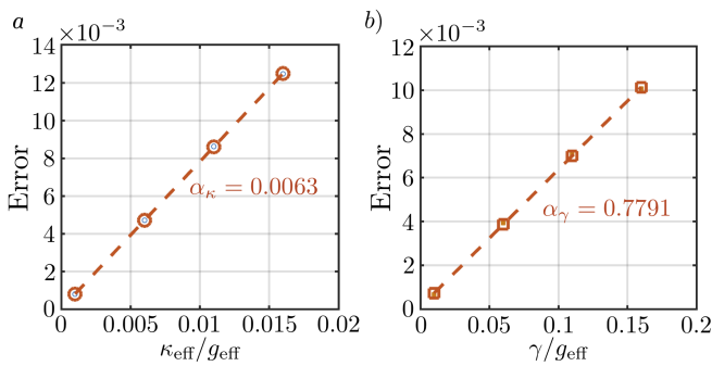
FIG. 8. Distribution of the fidelity error \varepsilon for the optimized detuning \Delta^* = \mathcal{J} as a function of a) \kappa/g_{\text{eff}} for \pi/T_2^* = 0 and b) \gamma/g_{\text{eff}} for \kappa = 0 . Each panel shows the numerically calculated points (square/circles) together with the linear interpolation (dashed line) with slope a) \alpha_\kappa and b) \alpha_\gamma .
