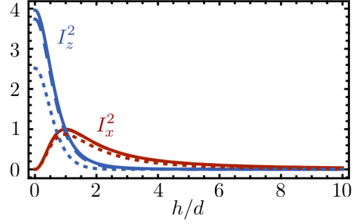
FIG. 4. Plot of the parameters I_z and I_x in function of h/d for l/d = 10 (dotted line), 10^2 (dashed line), 10^3 (solid line). For I_x the dashed and solid line are almost coincident.
