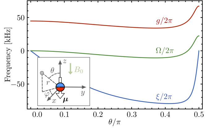
FIG. 7. Plot of the couplings \xi , g , and \Omega vs the position angle \theta . The remaining parameter have the following values: R = 350\text{nm} , r_0 = R + 20\text{nm} , B_0 = 70\text{mT} , and \gamma_0, \gamma_q as in the caption of Fig. 3. Inset: general configuration of the nanomagnet-qubit system.
