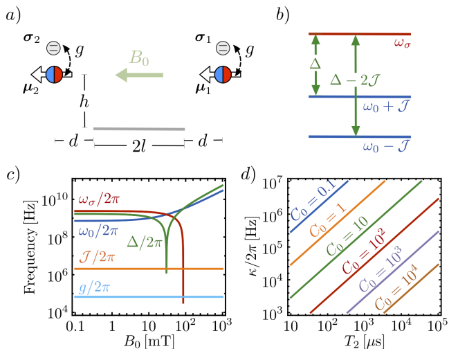
FIG. 3. a) Elementary HML configuration (single cell) with two identical spin qubits locally coupled to each magnetic particle. b) Level structure of the system, where \omega_0 \pm \mathcal{J} are the magnonic normal mode of the elementary cell. c) Relevant frequencies and coupling of the system in a) as a function of the applied field B_0 . d) Cooperativity C_0 as a function of the decoherence rates \kappa and \pi/T_2 for a fixed magnet-qubit coupling g . Other parameters: R = 350\text{nm} , r_q - R = 20\text{nm} , d - R = 100\text{nm} , l = 5\mu\text{m} , \tau = 50\text{nm} , h = 0 , \gamma_0 = 1.76199 \times 10^{11}\text{rad} \cdot \text{Hz} \cdot \text{T}^{-1} , \gamma_q = 1.76149 \times 10^{11}\text{rad} \cdot \text{Hz} \cdot \text{T}^{-1} , M_s = 196 \times 10^3 \text{T} \cdot \text{m}^{-3} (YIG saturation magnetization), and k_a = 2480 \text{J} \cdot \text{m}^{-3} (YIG anisotropy energy density). The parameters for YIG are taken from [51].
