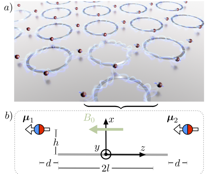
FIG. 1. a) Schematic illustration of a general hybrid magnetic lattice (HML) of superconducting-loops and magnetic particles. b) Scheme of the simplest cell of the HML: two magnetic particles positioned at a distance d and height h from two opposite points of a superconducting ring of radius l .
