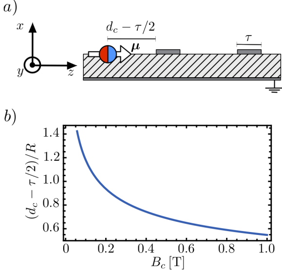
FIG. 5. a) Lateral view (not to scale) of a magnetic particle positioned on the substrate (hatched grey region) sustaining the superconducting-ring ( h = 0 ) at a distance d - \tau/2 from the closest point of the superconducting-ring wire (dark grey region) of thickness \tau . b) Critical distance d_c - \tau/2 in unit of R at which the field produced by the magnetic moment at the closest wire point equals B_c . Other physical parameters are taken from the caption of Fig. 3.
