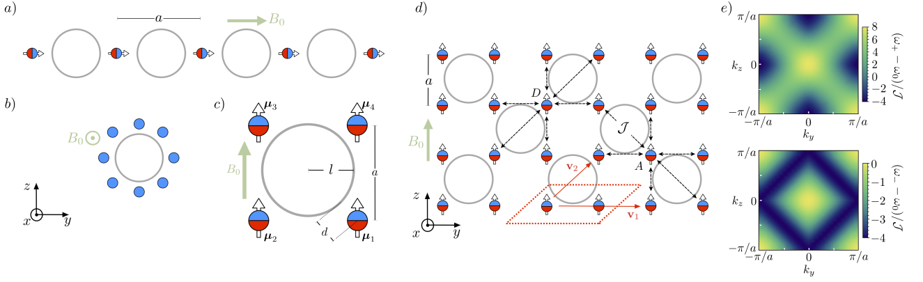
FIG. 2. a) Top view of a 1D HML. b) Top view of a system of vertically polarized magnets around a common loop. c) Unit cell of a 2D HML comprising one loop and four magnetic particles. d) Top view of a 2D HML implementing a 2D magnonic crystal by a checkboard arrangement of the single cell in c). The black dashed arrows indicate coupling between nearest-neighbors at the same rate \mathcal{J} and the red dashed area corresponds to the elementary cell of such a magnonic crystal with Bravais vectors \mathbf{v}_1 and \mathbf{v}_2 . e) Plot for the magnonic bands (\omega_{\pm} - \omega_0)/\mathcal{J} of the 2D HML in d).
