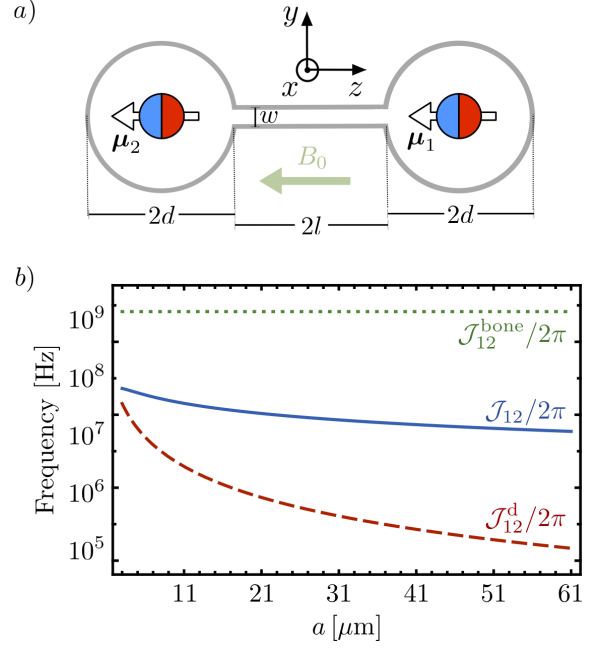
FIG. 6. a) Bone shape coil for enhancing the magnon tunneling rate between distant magnets. In such a configuration the total distance between the magnets is a = 2d + 2l . b) Magnon tunneling rate \mathcal{J}_{12} (solid blue line), \mathcal{J}_{12}^d (dashed red line), and \mathcal{J}_{12}^{\text{bone}} (dotted green line) as function of the magnets separation a . We assumed R = 1 \mu\text{m} , d = 500 \text{ nm} , and \tau = 50 \text{ nm} . The tunneling rate \mathcal{J}_{12} ( \mathcal{J}_{12}^d ) corresponds to the loop-mediated (free-space magnetic dipole) tunneling rate in the configuration shown in Fig. 1.b.
