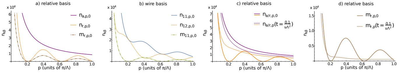
Figure 8. Distribution for a non-thermal initial state with parameters as in Table I and an oscillation length \xi = 7.5/\Lambda : a) The initial relative and absolute occupations and b) the intra- and inter-wire occupations. c+d) Time evolution of the relative and absolute density occupations in the presence of phonon-phonon collisions. The collisions lead to an adjustment of n_{r,p,t} and n_{a,p,t} as time evolves, which is accompanied with the temporal fade out of the scale \xi .
