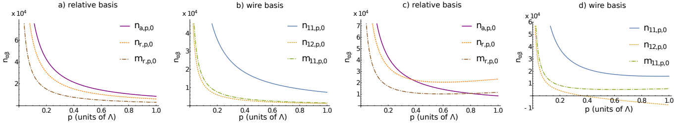
Figure 2. For parameters as in Table I but \chi_r set to zero \chi_r = 0 by hand: a) initial distribution in the absolute n_a and relative n_r, m_r modes, b) initial distribution in the single wire basis. We focus in this analysis on the low-energy dynamics of the system below a certain cutoff p < \Lambda . Due to equations (4.3) and (4.4), the initial distributions are almost thermal for all momenta. For parameters as in Table I but \chi_r = \frac{1}{4\pi\rho_0}K : c)+d) The presence of \sqrt{T_r/(\nu\chi_r)} \approx 0.5\Lambda < \infty distinguishes two momentum regimes: Small momenta |p| < \sqrt{T_r/(\nu\chi_r)} with a thermal relative density n_r = T_r/(\nu|p|) < n_a and large momenta |p| > \sqrt{T_r/(\nu\chi_r)} with a linear increasing density n_r = \chi_r|p| > n_a .
