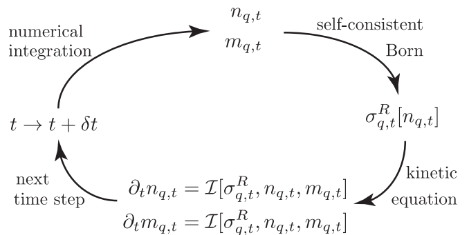
Figure 1. Schematic illustration of the numerical routine for solving the kinetic equations. For a given occupation n_{q,t}, m_{q,t} , the self-energies are computed within self-consistent Born approximation. Inserting the self-energies into the collision integral determines the evolution of n_{q,t}, m_{q,t} via the kinetic equation. Numerical integration yields the occupations at the next time step t \rightarrow t + \delta t .
