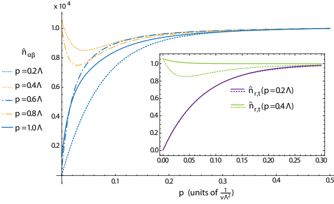
Figure 9. Long-time relaxation of the phonon densities n_{r,p,t} for momenta p = \frac{l\pi}{2\xi} \approx 0.2\Lambda for \xi = 7.5/\Lambda and l = 1, 2, \dots, 5 , as in Fig. 8 ( l = 2, 4 correspond to even modes in the experiment [16]). For better visualization, the phonon densities are normalized to their asymptotic, thermal value \hat{n}_{r,t}(p) = n_{r,p,t}\nu|p|/T_f . The relaxation can be described in terms of a two-stage process. In the first stage, the relative modes try to approach one common temperature \sim T_r < T_f in order to remove the oscillating structure in n_{r,p,t} , i.e. energy is redistributed within the relative modes. This can be achieved already by local scattering processes with momenta \sim \xi^{-1} . In the second, slower stage, the temperature between the relative and the absolute mode are adjusted via energy transfer from the absolute to the relative mode. The two stages are most prominently visible in the evolution for the momenta p = 0.4, 0.8\Lambda , which first decrease below their asymptotic value and then, together with the other modes, increase again towards T_f . The inset shows comparison of a bare exponential decay (bold lines) corresponding to a single stage relaxation process with the numerical data (dotted lines) for p = 0.2\Lambda (lower graphs) and p = 0.4\Lambda (upper graphs). For the latter, the deviation is very pronounced.
