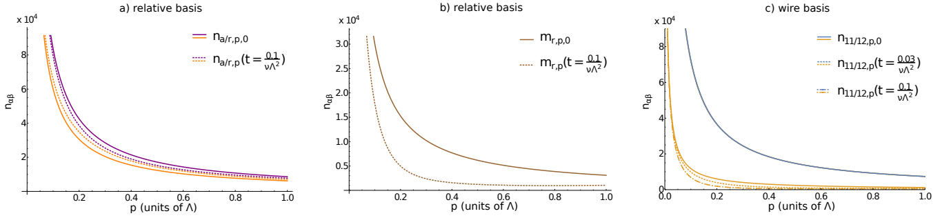
Figure 4. Parameters as in Table I but \chi_r = 0 : a) The relative and absolute phonon densities, n_{i,p} with i \in \{r, a\} , with an initial thermal distribution (bold lines) as shown in Fig. 2 approach each other as time evolves. Both occupations converge against a final thermal state characterized by a single temperature T_f . b) The anomalous density m_{r,p,t} decays in time and approaches zero. c) In this case, \chi_r \approx 0 is negligible and the evolution is governed by the slow decay of n_{12,p,t} in time, while n_{11,p,t} remains constant in time (all blue (dark) lines coincide).
