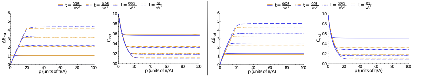
Figure 6. Relative phase fluctuation \Delta\theta_r and phase correlation function C for a nearly thermal initial state with \chi_r \approx 0 (left column, corresponding to data as in Fig. 4) and for an initial state with non-negligible linear tail \chi_r \neq 0 (right column, corresponding to data as in Fig. 5). The evolution in the absence (orange) and in the presence (blue) of phonon-phonon collisions is compared for increasing times t = (1, 2, 3, 4)/(40v\Lambda^2) .
