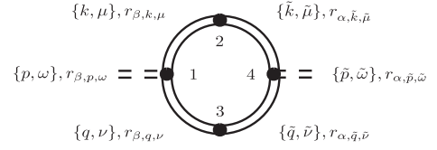
Figure A1. One-loop diagram for the self-energy \Sigma . Each line has momentum and frequency \{k, \omega\} and a direction r_{\alpha,k,\mu} = \pm 1 for outgoing, ingoing lines, which depends also on the wire index \alpha . Momentum conservation, energy conservation and the resonance condition have to be applied at each connecting element \{1, 2, 3, 4\} , which requires that normal (anomalous) self-energies are generated exclusively by normal (anomalous) Green's functions.
