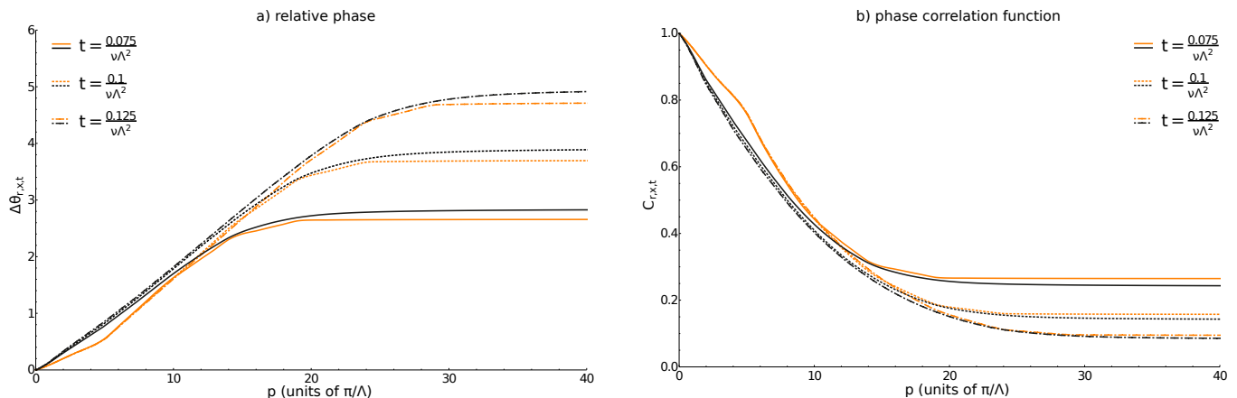
Figure 10. Initial parameters as in Table I and an oscillation length \xi = 7.5\Lambda^{-1} : a) Comparison of the evolution of the relative phase \Delta\theta_{r,x,t} in the presence (black (dark) lines) and absence (orange (bright) lines) of phonon collisions. b) The same comparison for the coherence factor C(x,t) . The difference between a thermal and a non-thermalized state becomes quite significant at distances on the order of twice the oscillation length, x = 2\xi .
