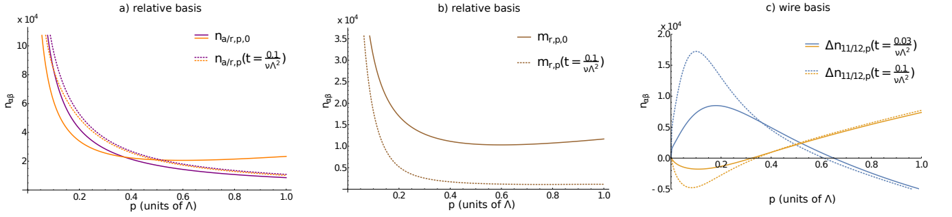
Figure 5. Parameters as in Table I with \chi_r = \frac{1}{4\pi\rho_0}K : a) The initial diagonal relative phonon density n_{r,p} (bright, bold) has a linear tail (see Fig. 2) and energy stored at larger momenta. During the time evolution, n_{r,p,t} and n_{a,p,t} converge towards an identical final distribution, which corresponds to a larger temperature. Energy is distributed from larger to small momenta. b) The off-diagonal occupation decays to zero exponentially in time. c) Time evolution of the difference \Delta n_{\alpha,p}(t) = n_{\alpha,p}(t) - n_{\alpha,p}(0) . The crossover momentum p_t^{(c)} separating fast, thermal-like evolution at p > p_t^{(c)} from a slow non-equilibrium relaxation at p < p_t^{(c)} leads to a bump in \Delta n_{\alpha,p}(t) as discussed in the main text.
