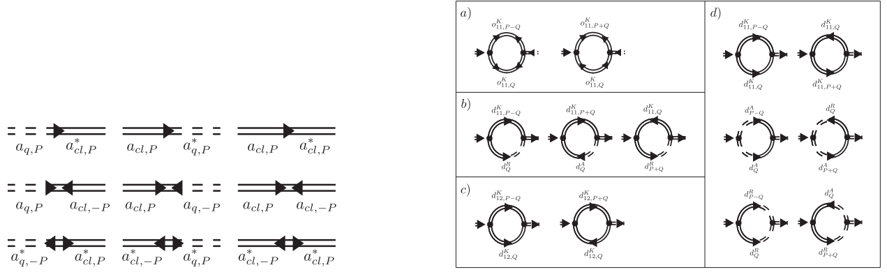
Figure A2. Left column: Illustration of the diagrammatic lines for the propagators in Keldysh space. Dashed lines correspond to quantum fields and bold lines to classical fields. Arrows indicate the momentum and energy transfer direction, going from annihilation to creation operators. Right column: Diagrammatic representation of the self-energy diagrams. a) Anomalous intra-wire Keldysh self-energy, b) Retarded self-energy, c): Normal inter-wire Keldysh self-energy, d): Normal intra-wire Keldysh self-energy.
