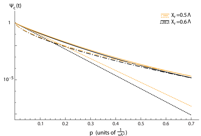
Figure 7. Time evolution of the coherence factor \Psi_c(t) from the kinetic equations (bold line) compared to an exponential decay \sim \exp(-t/t_0) (dashed line), as predicted from pure dephasing, and a stretched exponential \sim \exp(-(t/t_0)^{2/3}) (dash-dotted line), as predicted from phonon collisions, see Eqs. (4.16), (4.17). The colors (bright and dark) represent two different initial states with \chi_r = 0.5\Lambda^{-1} and \chi_r = 0.6\Lambda^{-1} .
