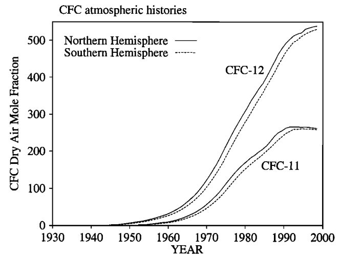
Figure 11. Reconstructed history of the atmospheric dry air mole fractions of CFC-11 and CFC-12 in the Northern and Southern Hemispheres. In effect, the Southern Hemisphere concentrations lag the Northern Hemisphere values by just over 1 year [from England , 1995].
