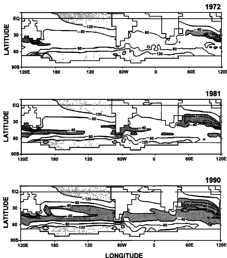
Figure 5. Maps of predicted \Delta^{14}\text{C} (per mil) at 755-m depth during 1972, 1981, and 1990 in the bomb-produced \Delta^{14}\text{C} simulation of Toggweiler et al. [1989b]. Carbon 14 values in excess of -40\text{‰} indicate the presence of bomb-produced ^{14}\text{C} .
