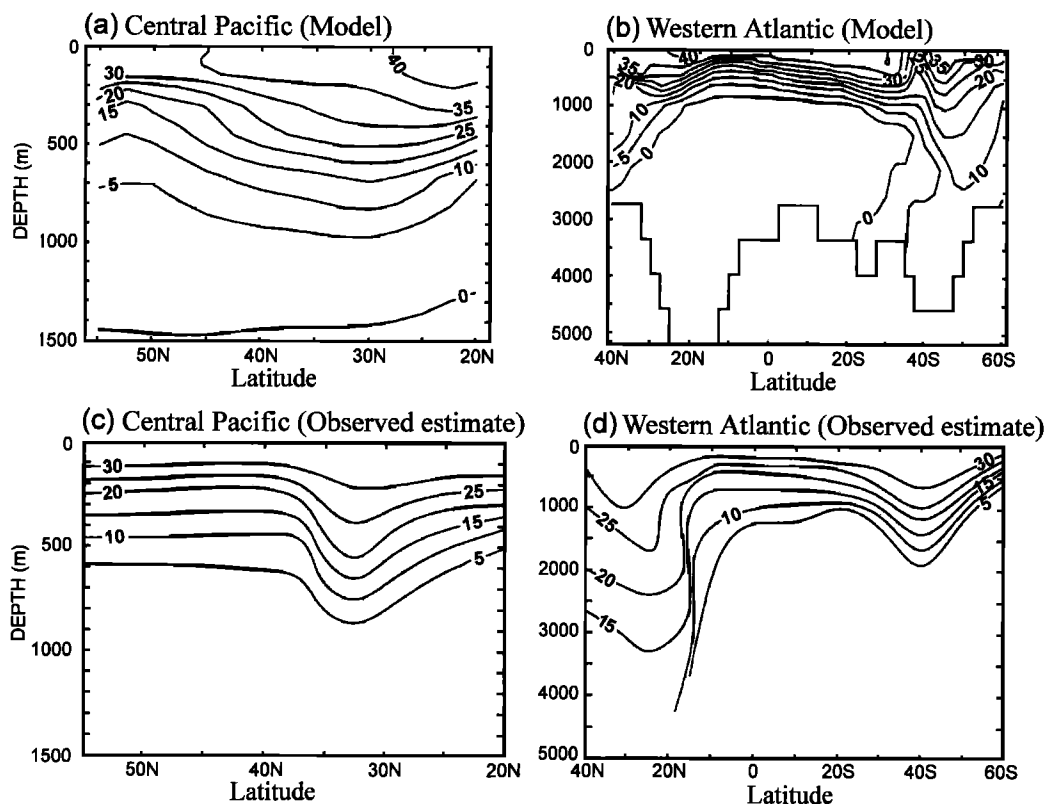
Figure 15. Simulated and observed estimates of the distribution of anthropogenic dissolved inorganic carbon (DIC) along the GEOSECS central Pacific and western Atlantic sections [from Taylor, 1995; and Chen, 1982a, 1982b]. Contour interval is 5 \mu\text{mol kg}^{-1} . It should be noted that considerable uncertainty remains in the observed estimates.
