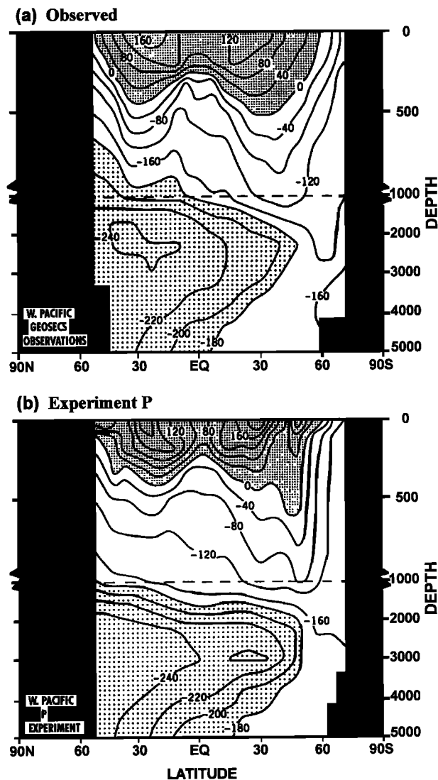
Figure 3. Western Pacific section of \Delta^{14}\text{C} (per mil) in (a) observations and (b) the bomb-produced \Delta^{14}\text{C} simulation P of Toggweiler et al. [1989b] during 1974. A clear anthropogenic signal of \Delta^{14}\text{C} is seen in this experiment compared with Toggweiler et al. [1989a] (Figure 2).
