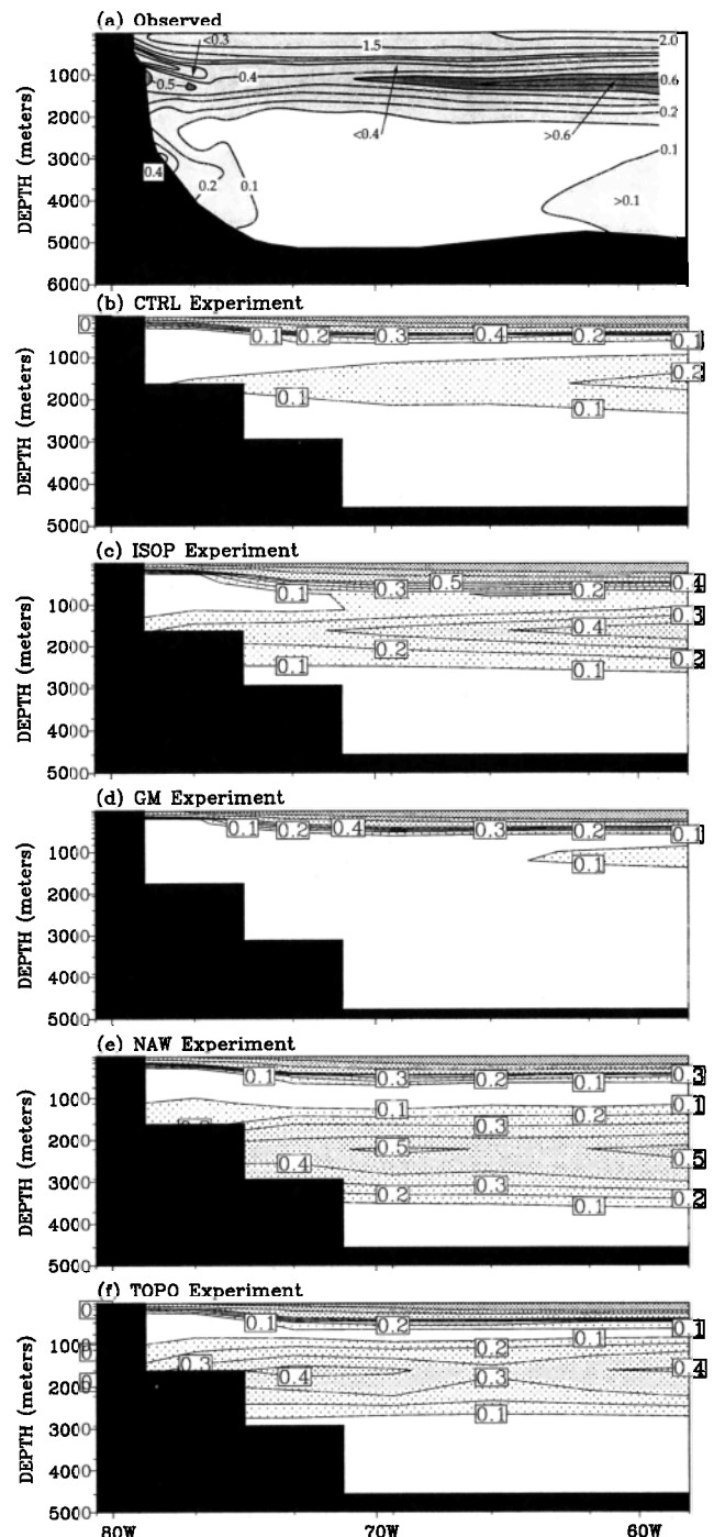
Figure 14. (a) Vertical section of observed CFC-11 along WBEX stations 22–38 near 32^\circ – 34^\circ\text{N} (redrafted from Smethie [1993] ). The WBEX section location is indicated in Figure 12a. CFC-11 concentrations greater than 0.1\text{ pmol kg}^{-1} are shaded. (b–f) Corresponding sections of simulated CFC-11 in each model case during April–May 1986 from England and Holloway [1998] . Contour levels are drawn at 0.1, 0.2, 0.3, 0.4, 0.5, 0.6, 1.0, 1.5, and 2.0\text{ pmol kg}^{-1} .
