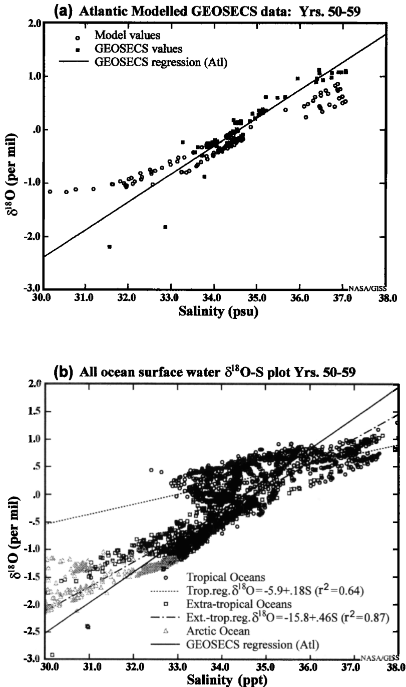
Figure 23. (a) Relationship between surface \delta^{18}\text{O} and salinity for GEOSECS data and the global model of Schmidt [1998]. (b) Relationship between \delta^{18}\text{O} and salinity for surface data points in the global model of Schmidt [1998]. Values are split into the tropical, extratropical and Arctic Oceans. Regression lines are fitted separately for each subregion. Also shown is the regression line for the GEOSECS Atlantic data.
