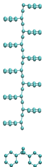
Figure 1.5.: Five different crystalline forms: two crystalline phases ( \alpha and \beta ) with trans-planar chains; three crystalline phases ( \gamma, \delta and \varepsilon ) with the s(2/1)2 helical chains.
