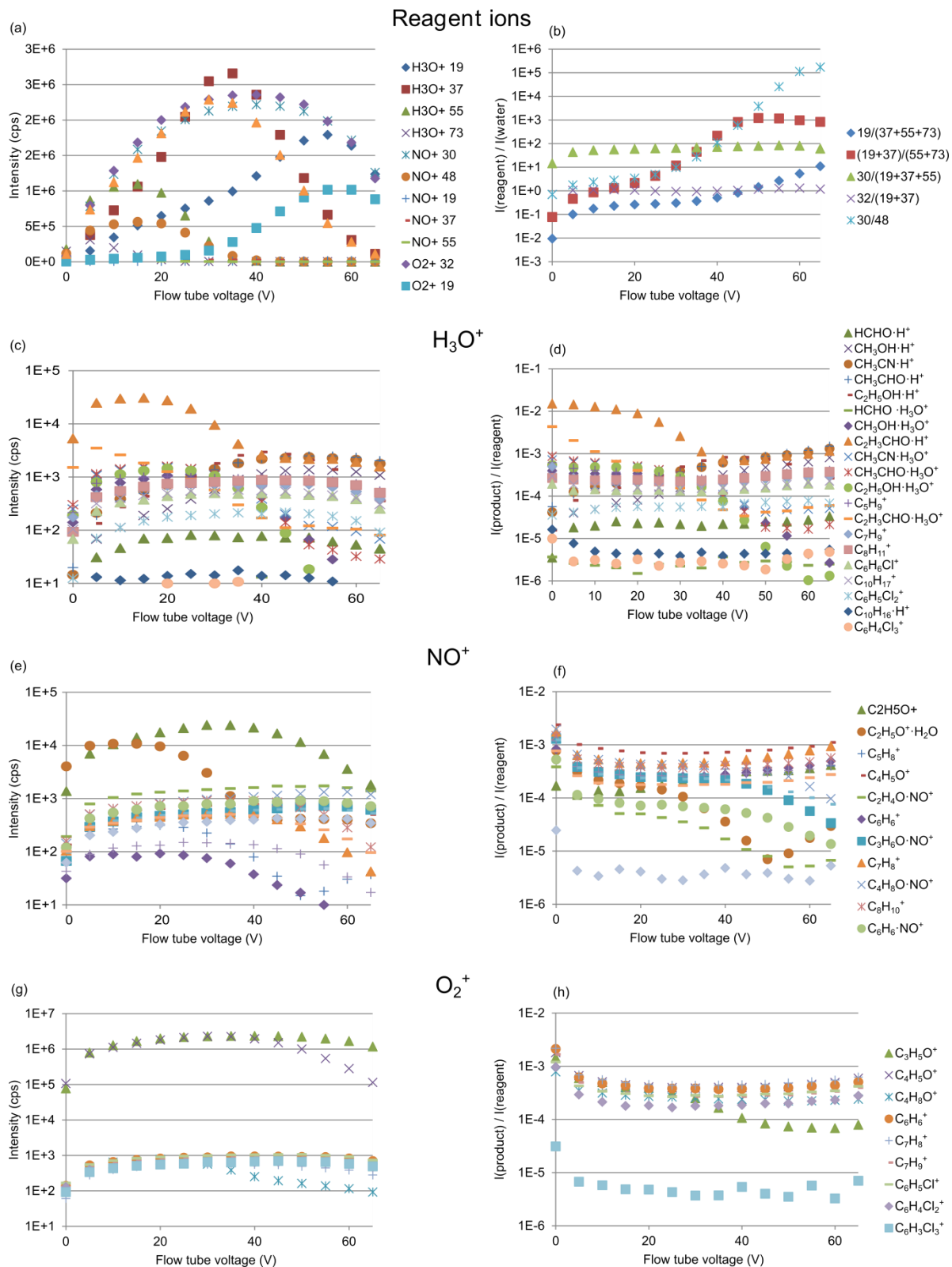
Figure S6: Flow tube voltage optimization for helium carrier gas and zero air dilution gas, \phi_{\text{FT}} = 395 \text{ sccm} , T_{\text{FT}} = 140^\circ\text{C} , 90% humidity at 25^\circ\text{C} . (a–b) for the different reagent ions H 3 O + , NO + , and O 2 + , the detected primary and secondary reagent ions symbolized by their mass as shown 19 = H 2 O + , 37 = H 3 O + ·H 2 O, 55 = H 3 O + ·2 H 2 O, 73 = H 3 O + ·3 H 2 O, 30 = NO + , 48 = NO + ·H 2 O, 32 = O 2 + . (a) absolute ion counts, (b) proportion of reagent ions relative to the water clusters. (c–h) behaviour of the product ions upon reaction with H 3 O + (19 + 37 + 55, c, d), NO + (e, f), and O 2 + (g, h) as reagent ions. (c, e, g) absolute ion counts, (d, f, h) counts normalized to reagent ion counts.
