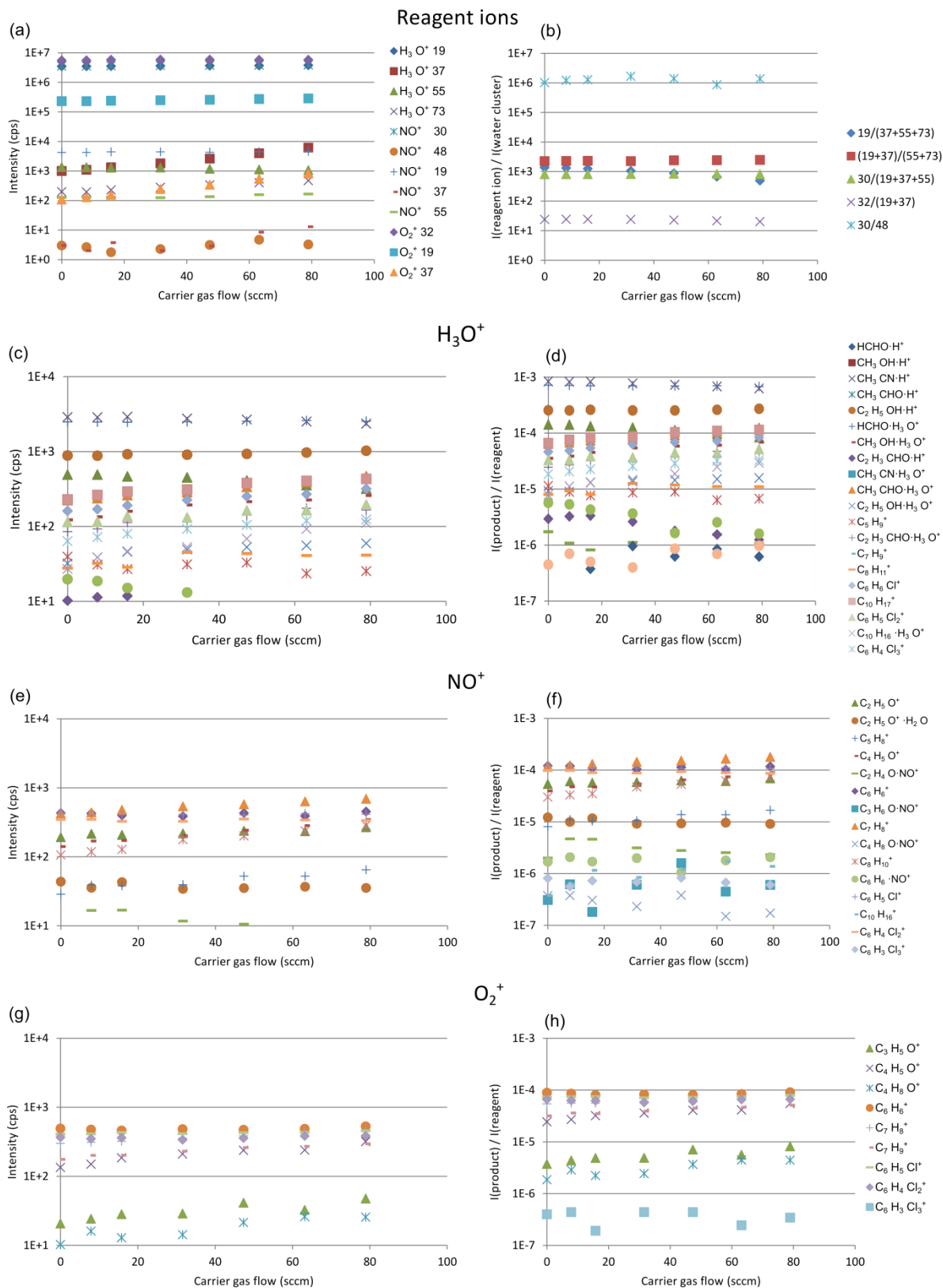
Figure S8: Carrier gas flow optimization for nitrogen carrier gas and zero air dilution gas, U_{\text{FT}} = 50 V, T_{\text{FT}} = 140^\circ\text{C} , 90% humidity at 25^\circ\text{C} , picture section of Fig. S7 for low carrier gas flows. (a–b) for the different reagent ions \text{H}_3\text{O}^+ , \text{NO}^+ , and \text{O}_2^+ , the detected primary and secondary reagent ions symbolized by their mass are shown 19 = \text{H}_2\text{O}^+ , 37 = \text{H}_3\text{O}^+\cdot\text{H}_2\text{O} , 55 = \text{H}_3\text{O}^+\cdot 2\text{H}_2\text{O} , 73 = \text{H}_3\text{O}^+\cdot 3\text{H}_2\text{O} , 30 = \text{NO}^+ , 48 = \text{NO}^+\cdot\text{H}_2\text{O} , 32 = \text{O}_2^+ . (a) absolute ion counts, (b) proportion of reagent ions relative to the water clusters. (c–h) behaviour of the product ions upon
