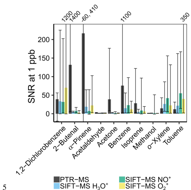
Figure S19: Signal to noise ratio (SNR) at 1 ppb ( \pm 95 % CI, df = 7) of PTR-MS and the different SIFT-MS reagent ions for different VOCs at 30 % humidity. The values above the biggest error bars resemble the values of the confidence intervals out of the depicted range. The high positive confidence interval is due to the high relative error of the blank.
