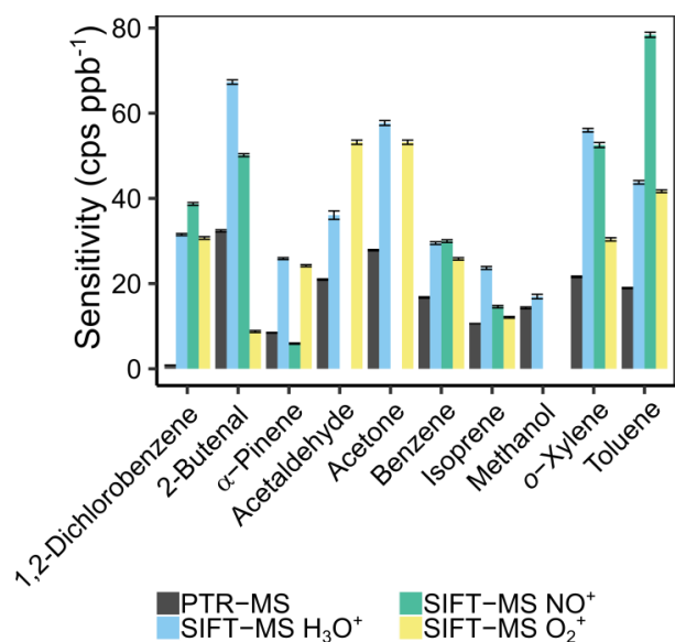
Figure S18: Instrument sensitivity \pm 95 % confidence interval (df = 26) of PTR-MS and the different SIFT-MS reagent ions for different VOCs at 30 % humidity. Sensitivity is defined here as the slope of the calibration curve.
