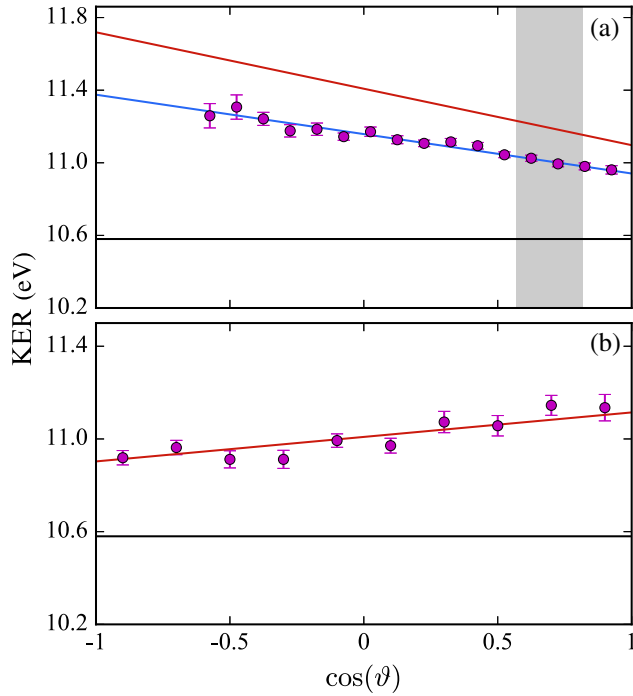
FIG. 2. Position of the maximum in the KER distribution between 10 and 12 eV for Compton scattering and K -shell photoionization of N_2 at h\nu = 40 keV as a function of \cos \vartheta , where \vartheta is the angle (a) \vartheta_{k_{ep}, k_{\gamma}} or (b) \vartheta_{k_{eA}, k_{sum}} . See the text for an explanation (including of the shaded area). Black lines, the KER peak position for Compton scattering ( KER_0 ); magenta points, measured data for the KER peak position for K -shell photoionization; red lines, expectation for \Delta KER + KER_0 , where \Delta KER is taken from (a) Eq. (3) or (b) Eq. (4); blue line, 0.7 \times \Delta KER + KER_0 [expectation from Eq. (3), assuming that only 70% of the maximum recoil energy is imparted on the ionic fragments].
