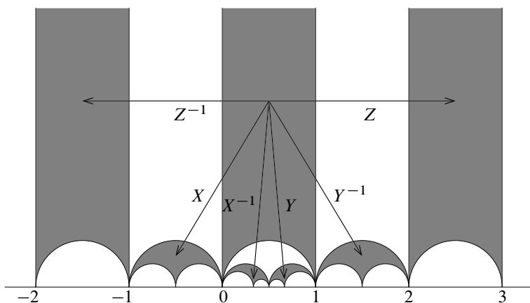
Figure 4. The action of the elements X^{\pm 1}, Y^{\pm 1}, Z^{\pm 1} \in \text{PSL}(2, \mathbb{Z}) on a triangle \mathcal{T} with vertices 0, 1, \infty of the Farey tessellation.
