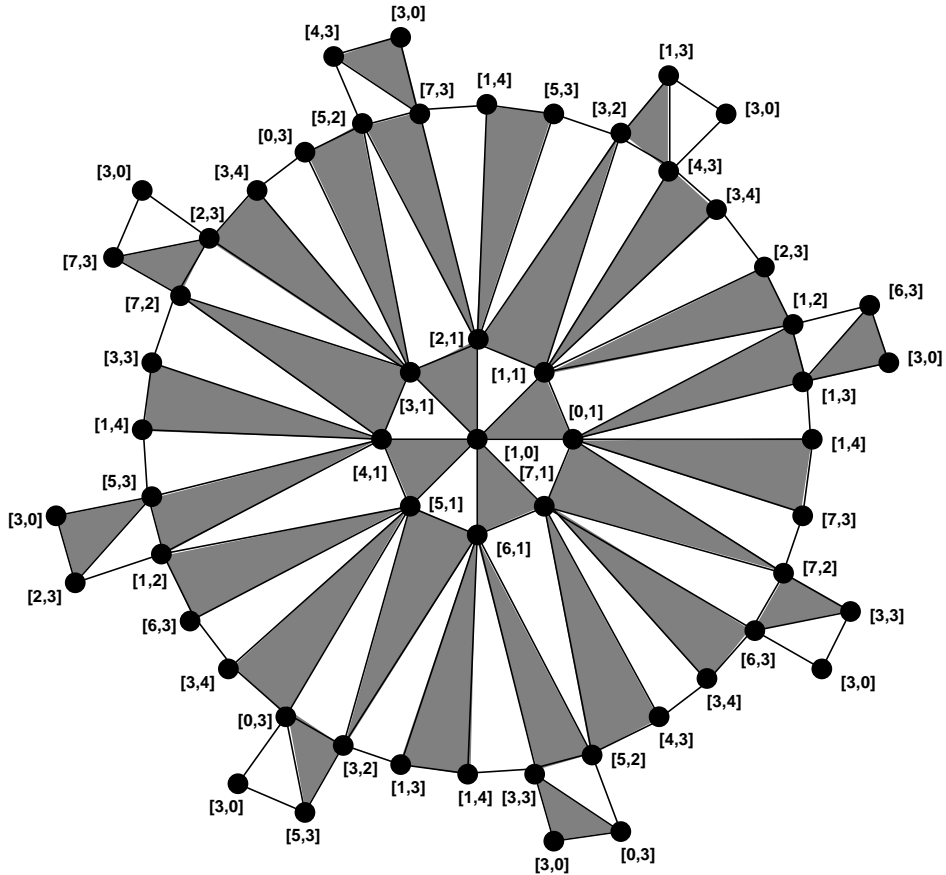
Figure 2. The Platonic graph \Pi_8 . Each triangle corresponds to a hyperbolic (\pi/4, \pi/4, \pi/4) -triangle of the tessellation of S(\Pi_8) . The edges along the boundary path are pairwise glued to obtain S(\Pi_8) .
