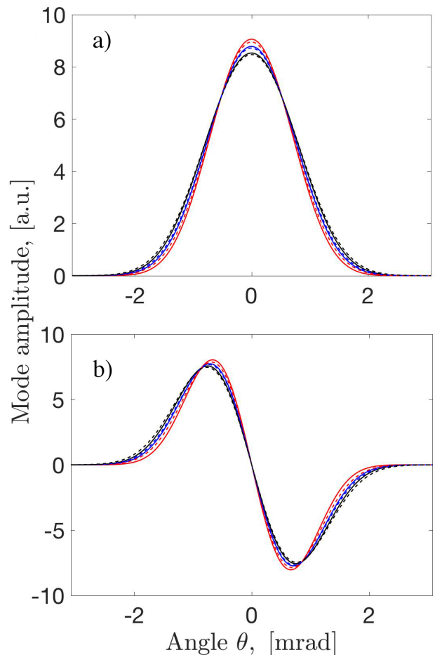
FIG. 5. a) The first and b) the second Schmidt modes for different parametric gain values: G=5.0 (red), G=5.7 (blue), G=6.6 (black). Solid lines represent theoretical calculations. Dashed lines stand for modes retrieved from the experiment.
