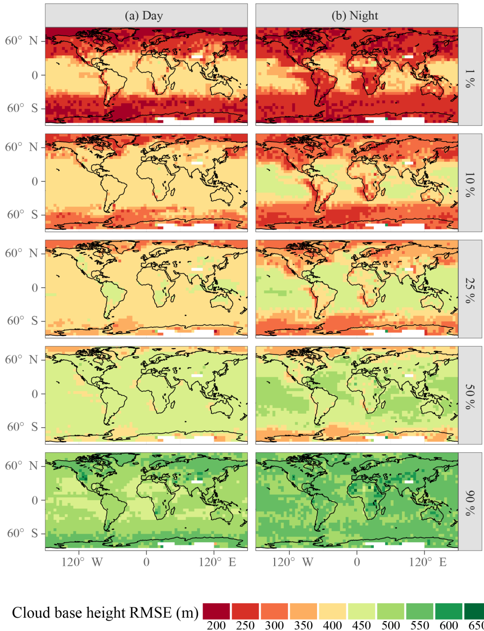
Figure 13. Cloud base uncertainty quantiles. Statistics are calculated within each 5^\circ \times 5^\circ latitude–longitude box. Panels (a) and (b) show statistics of daytime and nighttime retrievals, respectively; daytime and nighttime are defined by the CALIOP VFM product.
