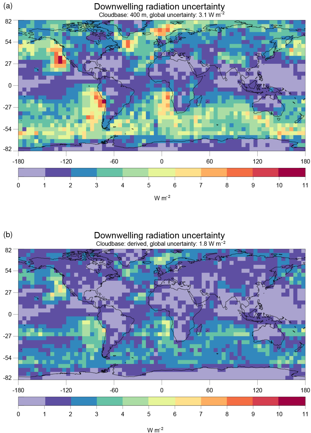
Figure 14. Uncertainty on the surface downwelling longwave radiation F_{\text{surf}}^{\downarrow} under two assumptions of z uncertainty: (a) constant 400 m uncertainty globally and (b) uncertainty achievable by selecting a high-quality subset of CBASE z .
