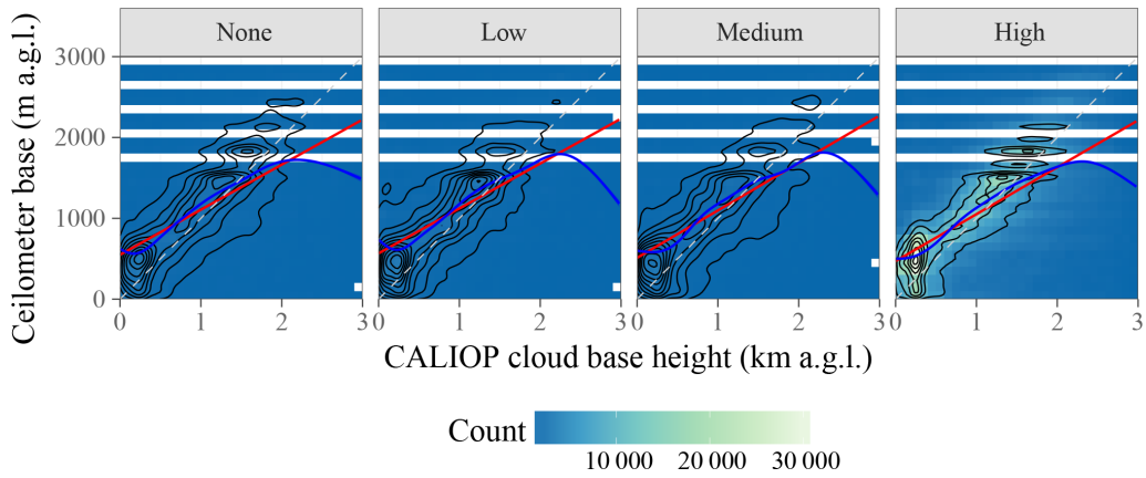
Figure 4. As in Fig. 3, but applying all requirements listed in Sect. 3.3.
