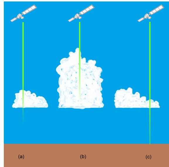
Figure 2. Schematic of CALIOP cloud base determination and evaluation strategy. In optically thick clouds (a, b), the lidar attenuates significantly within the cloud, rendering the cloud base information unreliable. However, z of thin clouds (c) can be used as a proxy for thick clouds in a cloud field with homogeneous z .
