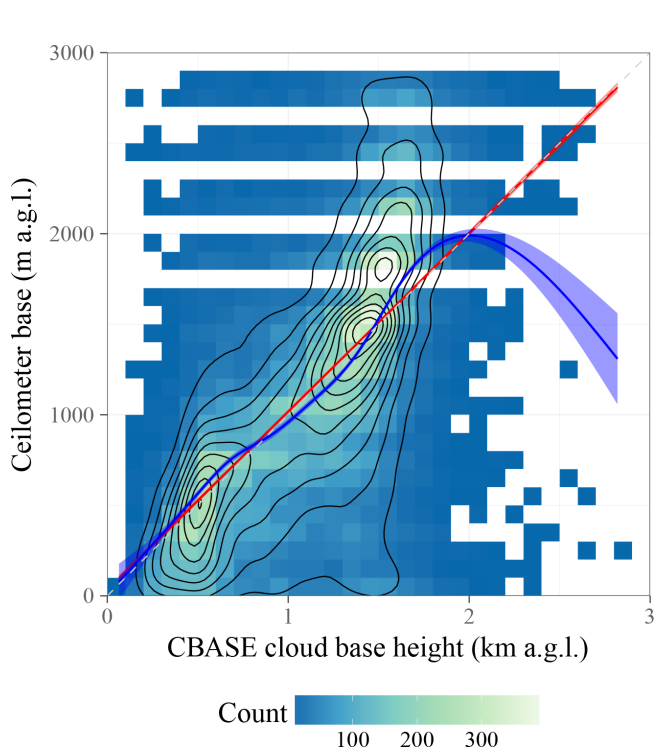
Figure 7. Scatter plot of CBASE versus ceilometer z for all A-Train overpasses over the contiguous US available for 2007; for description of the plot elements, see Fig. 3. The linear fit has a slope of 0.98 and an intercept of 33.96 m.
