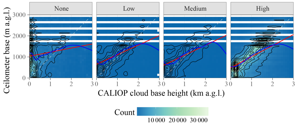
Figure 3. Scatter plots of CALIOP versus ceilometer cloud base height faceted by the CALIOP VFM QA flag; all CALIOP profiles meeting the temporal and spatial collocation requirements with a METAR enter into this plot. Color indicates the number of CALIOP profiles within each bin of ceilometer and CALIOP z ; black lines are contours of the empirical joint probability density; the red line is a linear least-squares fit, with the 95 % confidence interval shaded in light red; the blue line is a generalized additive model regression (Wood, 2011), with the 95 % confidence interval shaded in light blue (due to the large dataset, the line width exceeds the confidence intervals in these plots); the dashed gray line is the one-to-one line. Statistics of the relationship between CALIOP and ceilometer base heights are provided in Table 2.
