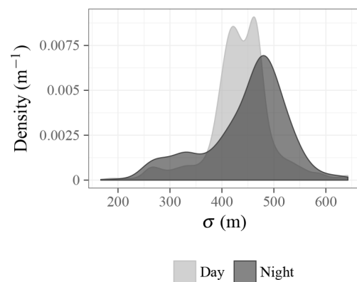
Figure 12. Distribution of predicted z uncertainty \sigma .
