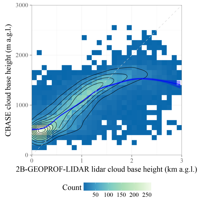
Figure 10. Scatter plot of 2B-GEOPROF-LIDAR lidar-only versus CBASE z . For description of the plot elements, see Fig. 3; because both cloud base measures have comparable uncertainty, linear regression is a misleading diagnostic (Pitkanen et al., 2016) and has not been included. The mean difference between 2B-GEOPROF-LIDAR and CBASE is 0.05 km, the root-mean-square difference is 0.41 km, and the correlation coefficient is 0.79.
