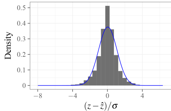
Figure 8. Distribution function of cloud base error divided by predicted uncertainty; for the ideal case of unbiased z and unbiased uncertainty, the distribution would be Gaussian with zero mean and unit standard deviation. The superimposed least-squares Gaussian fit (blue line) has a mean of 0.04 and standard deviation of 1.06.
