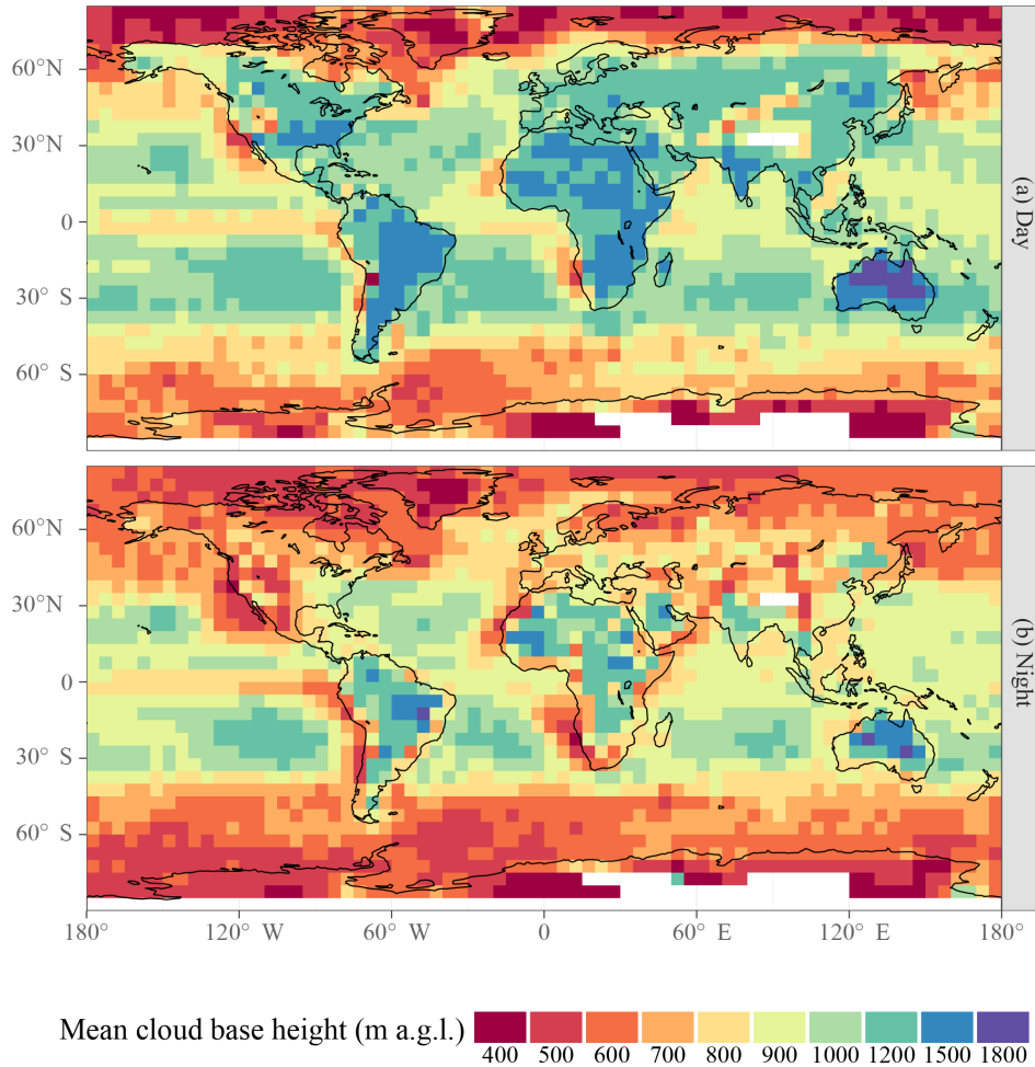
Figure 11. Geographic distribution of mean z above ground level. Statistics are calculated within each 5^\circ \times 5^\circ latitude–longitude box and separately for CALIOP daytime (a) and nighttime (b) overpasses.
