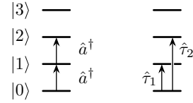
FIG. 1. Two types of excitation operators for a bosonic degree of freedom. Both can be used to access any number state, and both are sets of commutative operators. But the operators \hat{\tau}_n are additionally nilpotent, simplifying CC formulations that use this form.
