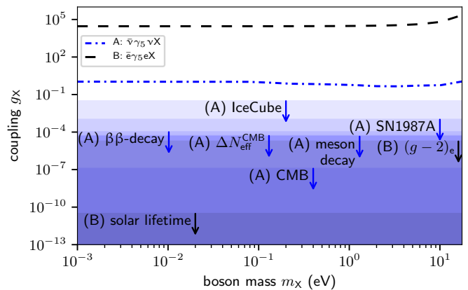
FIG. 7. Statistical sensitivity contours for eV-scale light pseudoscalar bosons - Shown is the 90% C.L. statistical sensitivity of KATRIN for the detection of eV-scale light pseudoscalar bosons. The types A, B are defined according to Tab. I. Furthermore, the shaded areas mark the parameter regions allowed from constraints discussed in Sec. V.
