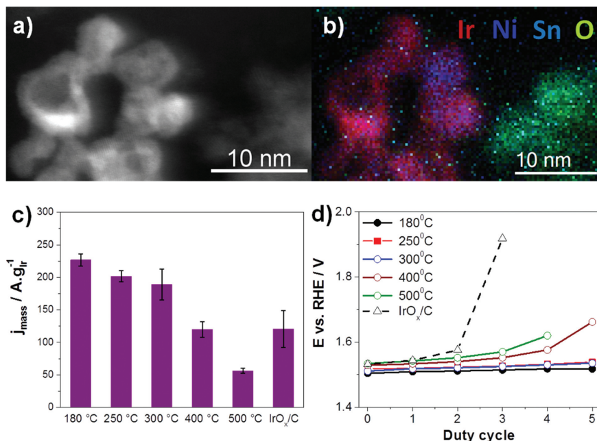
Fig. 4: (a) HAADF-STEM image of the \text{IrNiO}_{3.3}/\text{Meso-ATO-180} core-shell NP catalyst synthesized from PA- \text{IrNi}_{3.3}/\text{Meso-ATO-180} . (b) Elemental mapping of Figure 4a (Ir red, Ni blue, Sn dark cyan, O green). (c) Ir-mass-based activity at \eta = 300 \text{ mV} overpotential of \text{IrO}_x/\text{C} and \text{IrNiO}_{3.3}/\text{Meso-ATO-T} . (d) Potential at 1 \text{ mA cm}^{-2} using linear sweep voltammetry after duty cycles of \text{IrO}_x/\text{C} and \text{IrNiO}_{3.3}/\text{Meso-ATO-T} . Temperature (T) at which NPs have been treated is given for each data set. Measurement conditions: 0.05 \text{ M H}_2\text{SO}_4 , 1600 rpm. The loading of Ir was 10.2 \text{ mg cm}^{-2} . Adapted with permission [43].
