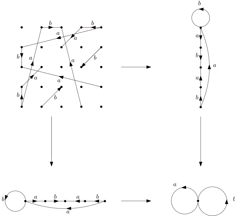
FIGURE 2. Only non-diagonal components of the fiber product are drawn.
