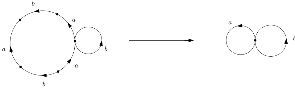
FIGURE 1. The immersion f : A \rightarrow X .
