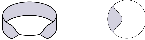
Figure 1.1: A pair of degenerate annuli, one (from [Hen14]) depicted in three space, and another embedded in the complex plane.
