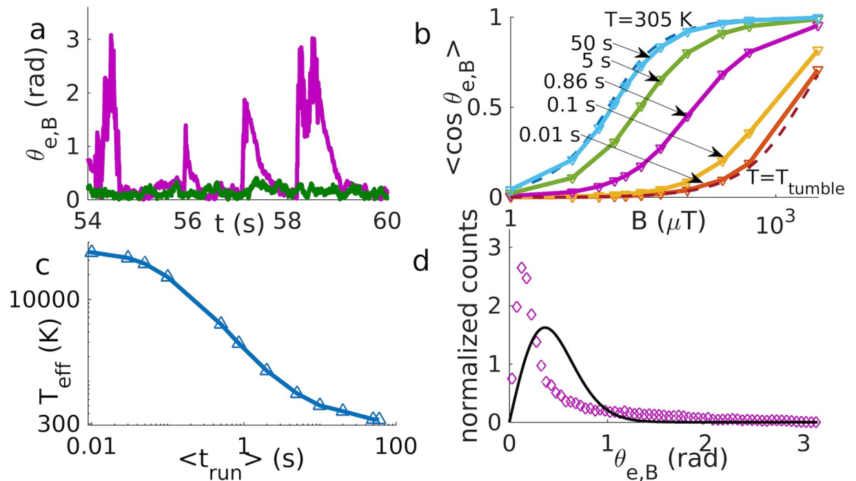
Fig 3. Motion with magnetic torque. a) Alignment angle vs. time for run and tumble (in purple) and run and reverse (in green) for a mean run time of 0.86 s at 500 \mu T. b) Langevin plots for run and tumble compared to theoretical Langevin functions at T and T_{tumble} (dashed lines). Each line corresponds to a different mean run time. c) The effective temperature obtained by the Langevin fit in b) is plotted against the mean run time. d) The distribution of the alignment angle for run and tumble with a mean run time of 0.86 s at 500 \mu T (data points) deviates from the thermal distribution with the corresponding effective temperature, 2896K (solid line).
