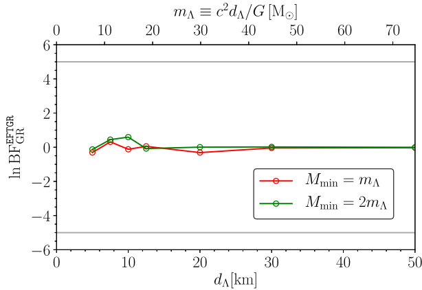
FIG. 5. The natural logarithm of the Bayes factors of the EFTGR versus GR waveform for GW170608 in the regime where d_\Lambda \lesssim M , with M the mass of either BH in the binary, with corresponding m_\Lambda shown in the top x axis, when using the PN waveform model. We fix the minimum mass M_{\min} in the priors for the BH masses such that d_\Lambda < M is always satisfied in the GW template. To account for the systematic uncertainty in the validity of the waveform model, we use different values for the minimum mass in the prior M_{\min} as shown by the different curves.
