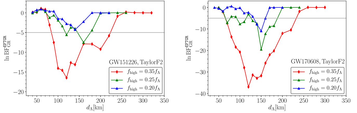
FIG. 3. The natural logarithm of the Bayes factor of the EFTGR versus GR waveform model for different choices of d_\Lambda (in km) when using the inspiral-only PN waveform model. We use different values for f_{\text{high}} when computing the likelihood function (4.8) to account for the different systematic uncertainties mentioned in the text. To compute f_\Lambda , we use the median source’s frame total masses obtained with IMR templates as reported in Refs. [40,41]. We show the results for the two lowest-mass GW events detected so far: GW151226 with total mass M_{\text{tot}} \simeq 22 M_\odot (left panel) and GW170608 with total mass M_{\text{tot}} \simeq 19 M_\odot (right panel). For reference, we mark the threshold \ln B_{\text{GR}}^{\text{EFTGR}} = -5 with a grey solid curve.
