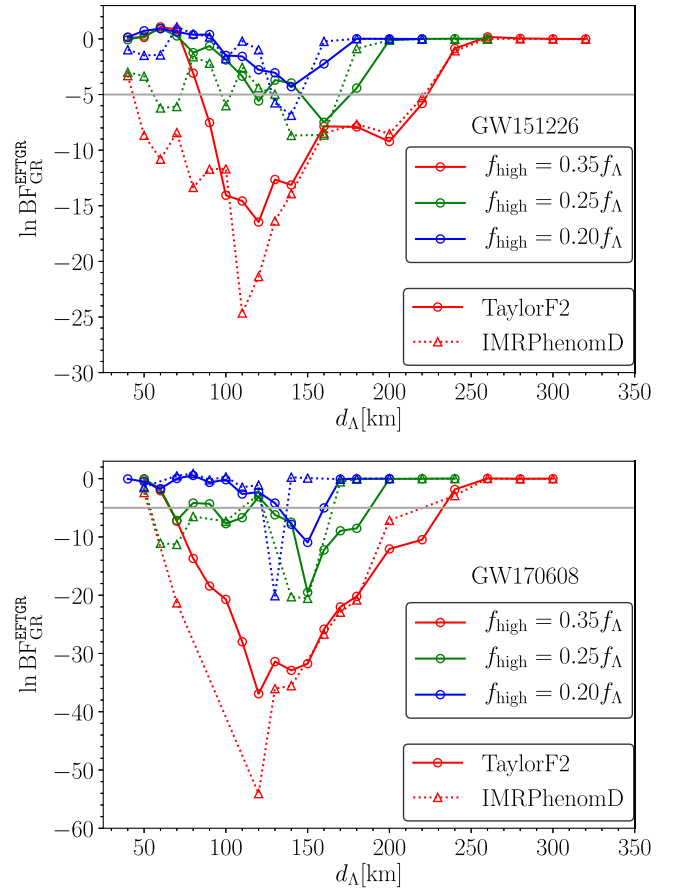
FIG. 6. Same as Fig. 3, but also showing the case where we use an IMR waveform model (IMRPhenomD). For the IMR model, the EFTGR correction is taped at the merger frequency that we take to be the peak of the waveform’s amplitude
