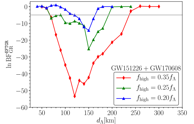
FIG. 4. The log Bayes factors of the EFTGR versus GR waveform when combining the results shown in Fig. 3.
