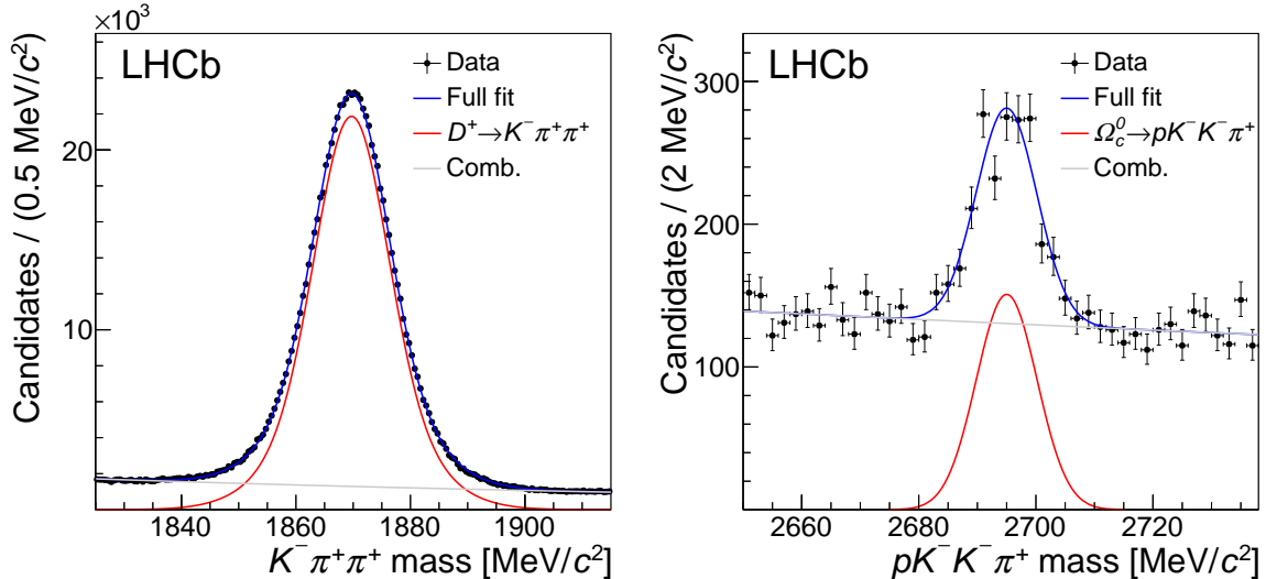
Figure 1: Invariant-mass distributions for (left) D^+ candidates in B \rightarrow D^+ \mu^- \bar{\nu}_\mu X decays and (right) \Omega_c^0 candidates in \Omega_b^- \rightarrow \Omega_c^0 \mu^- \bar{\nu}_\mu X decays. The results of the fits, as described in the text, are overlaid.
