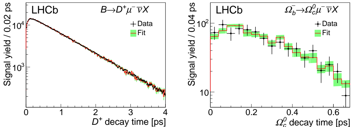
Figure 2: Decay-time spectra for (left) D^+ signal in B \rightarrow D^+ \mu^- X events and (right) \Omega_c^0 signal in \Omega_b^- \rightarrow \Omega_c^0 \mu^- X events. Overlaid are the fit results, as described in the text, along with the uncertainties due to finite simulated sample sizes.
