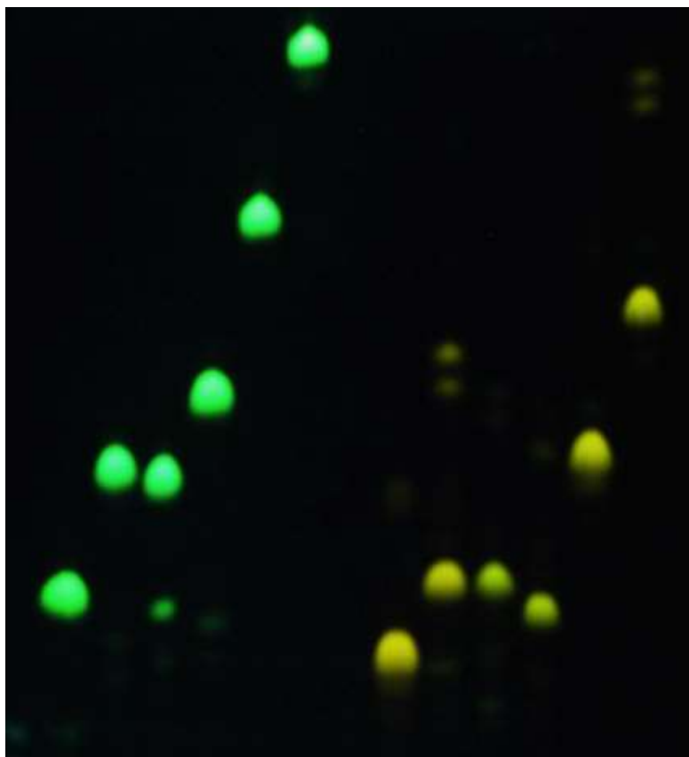
Figure S6. Gel electrophoresis of APTS conjugates with mannose and its oligomers (left part, green spots) and conjugates of dye 16 with mannose and its oligomers (right part, yellow spots); migration from “north” to “south”, pH 8.3. For structures, see Scheme S1 and the previous section ( Characterization of Conjugates ). Left part, green spots, from left to center: APTS+M, APTS+M 2 -2O, APTS+M 2 -3O, APTS+M 2 -4O, APTS+M 3 and APTS+M 4 . Right part, yellow spots, from center to right: 16 +M, 16 +M 2 -4O, 16 +M 2 -2O, 16 +M 2 -3O, 16 +M 3 and 16 +M 4 . Bands were detected by emission (excitation at 365 nm). Note that APTS+M 2 -2O moves a bit slower than APTS+M 2 -3O, 16 +M 2 -2O and 16 +M 2 -4O are undistinguishable, APTS+M 2 -4O moves much slower than other dimers, 16 +M 2 -3O moves faster than 16 +M 2 -2O or 16 +M 2 -4O.
