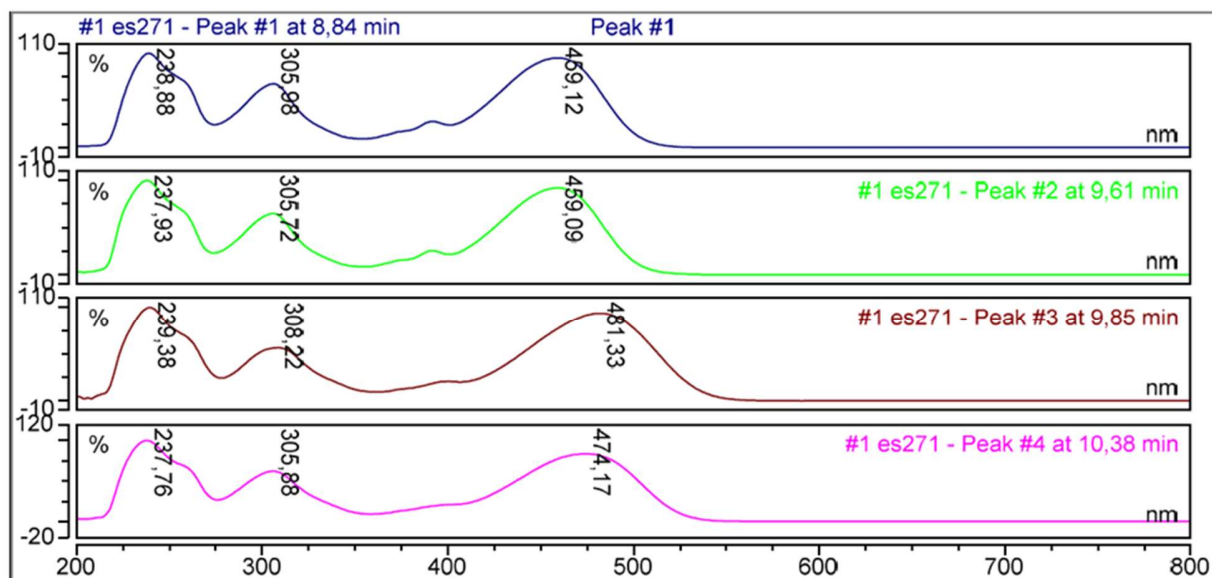
Figure S2. Step 1: dye 6-H , glucose and malonic acid were mixed and shaken at 40 °C for 1 h. Then the reaction mixture was dried. Starting material ( t_R = 10.3 , \lambda_{\text{max}} = 474 nm, magenta line, last spectrum) and Schiff base ( t_R = 8.8 , \lambda_{\text{max}} = 459 nm, dark blue line, first spectrum) were observed.
