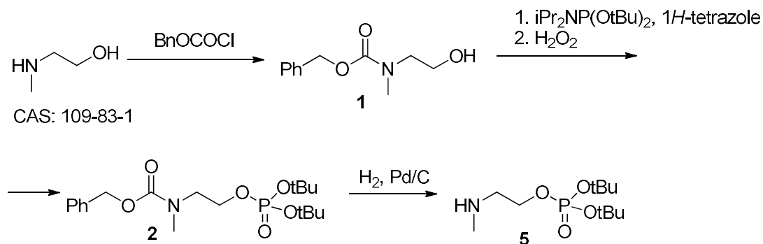
Scheme S1. Synthesis of 2-(methylamino)ethyl di(t-butyl)phosphate
