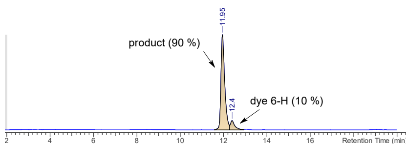
Figure S4. HPLC analysis of the reductive amination of 6-H with maltoheptaose (G 7 ) showed the conversion to glycoconjugate (detection at the isosbestic wavelength of 484 nm).
