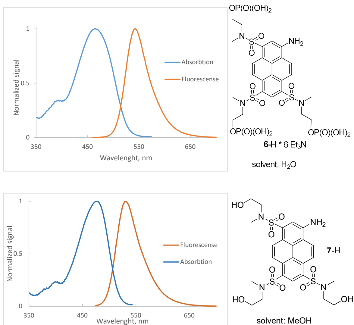
Figure S1. Absorption and emission spectra of pyrene dyes (see also Table 1 in the main text)
