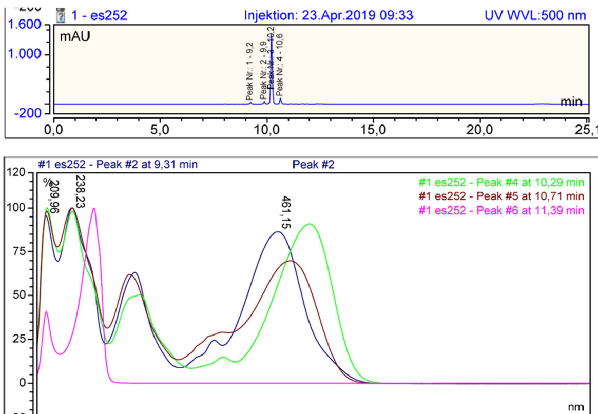
Figure S3. Step 2: 2-picoline-borane complex was added and the reaction mixture was shaken at 40 °C for 16 hours. Only traces of the starting material ( t_R = 10.7 min, \lambda_{max} = 471 nm, brown line) and Schiff base ( t_R = 9.3 min, \lambda_{max} = 461 nm, dark blue line) were observed. The main peak with t_R = 10.2 min represents the desired product ( \lambda_{max} = 496 nm, green line).
