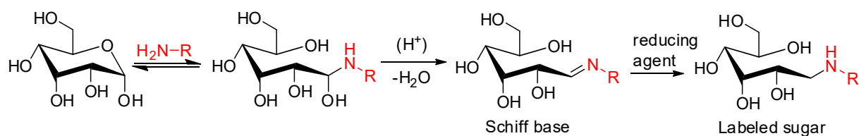
Scheme S3. Reductive amination of glucose
