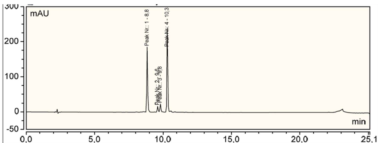
Scheme S3. Reductive amination of glucose
