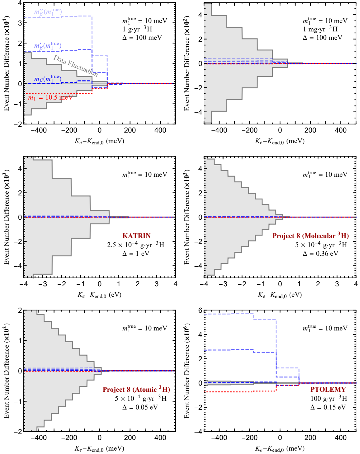
Figure 3: The difference of event numbers for the effective spectrum d\Gamma_{\text{eff}}/dK_e and the exact one d\Gamma'_{\text{cl}}/dK_e . The data are simulated by taking m_1^{\text{true}} = 10 meV. The blue histograms signify the event number deviations of the effective spectra from the exact one, whereas the gray filled histograms stand for the statistical fluctuations. Two nominal experimental setups have been assumed in the upper two panels, and in the remaining four panels we illustrate the cases of realistic experiments including KATRIN, Project 8 with molecular tritium and with atomic one, and PTOLEMY. Note that different scales on the axes have been adopted for each plot.
