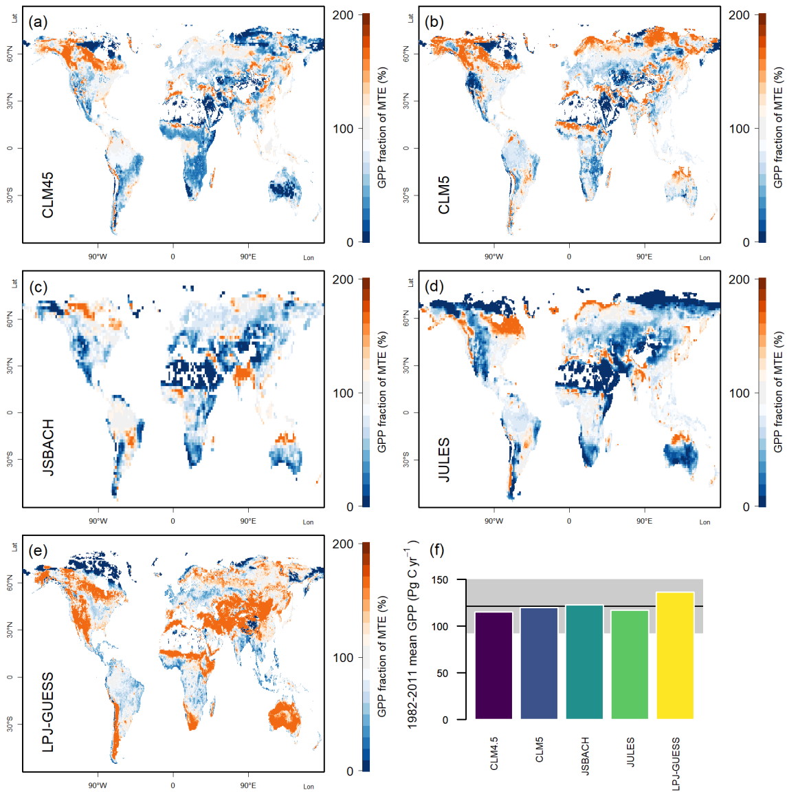
SI Fig. 2 Model output of 1982-2011 mean gross primary productivity (GPP). (a) – (e) Model estimates, shown as a percentage of the corresponding observation-based estimate (MTE) published by Jung et al. (2011). (f) Globally integrated estimates. Black line indicates the global average from the observation-based source; grey area indicates the globally integrated standard deviation from the global average in the model tree ensemble applied to obtain the global average.
