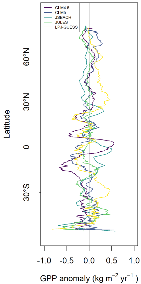
SI Fig. 1 Model output of 1982-2011 mean gross primary productivity (GPP) averaged by latitude, shown as the anomaly of the corresponding observation-based estimate (MTE) published by Jung et al. (2011).
