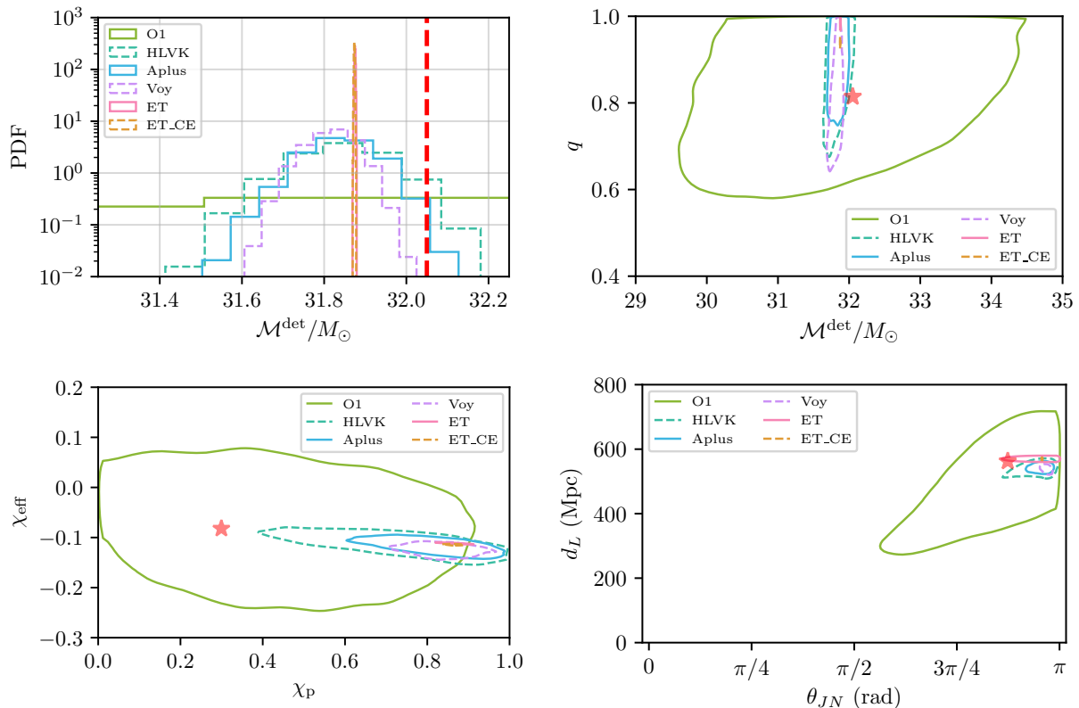
FIG. 3. Posterior PDFs for the SXS_BBH_0308 PN-NR hybrid signal (see Table I) using IMRPhenomPv2 as the template waveform for a sequence of detector networks (see Table II). We show either histograms of 1-dimensional PDFs or contours indicating 90% credible regions for 2-dimensional PDFs. Top left panel : histograms for detector-frame chirp mass Top right panel : contours for chirp-mass and mass-ratio Bottom left panel : contours for effective precession spin \chi_p and effective aligned spin \chi_{\text{eff}} Bottom right panel : contours for inclination angle \theta_{\text{JN}} and luminosity distance d_L . True parameter values of the source binary are indicated as red dashed lines or a red asterisk.
