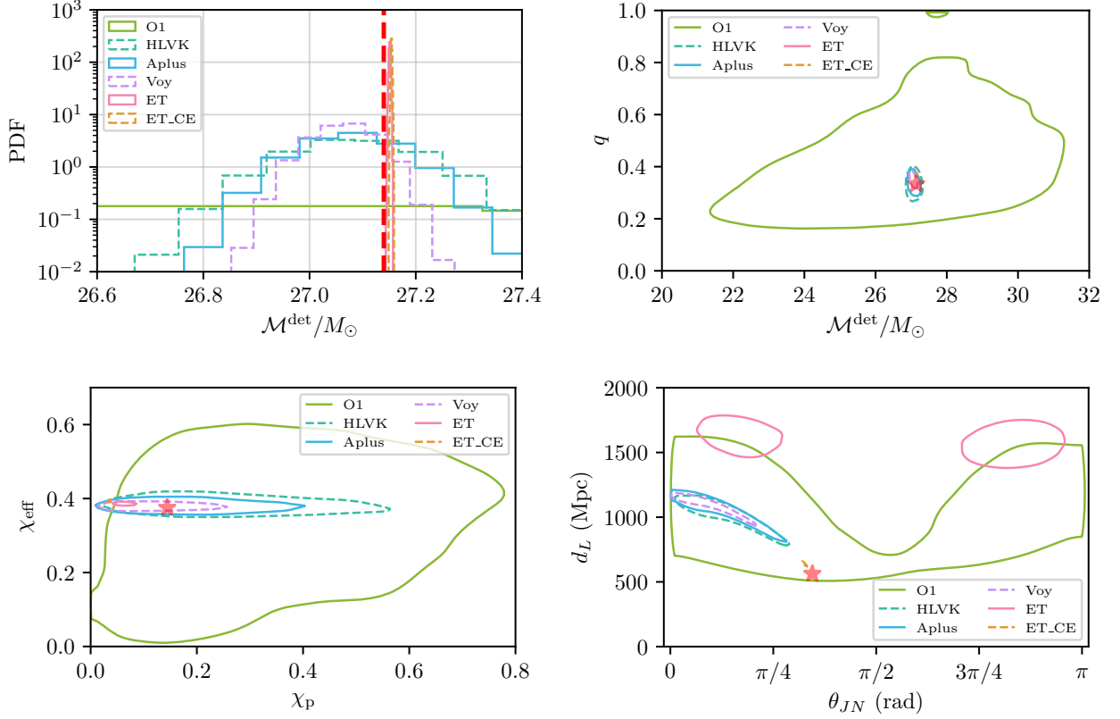
FIG. 4. Posterior PDFs for the SXS_BBH_0104 PN-NR hybrid signal (see Table I) using IMRPhenomPv2 as the template waveform for a sequence of detector networks (see Table II). We show either histograms of 1-dimensional PDFs or contours indicating 90% credible regions for 2-dimensional PDFs. Top left panel: histograms for detector-frame chirp mass Top right panel: contours for chirp-mass and mass-ratio Bottom left panel: contours for effective precession spin \chi_p and effective aligned spin \chi_{\text{eff}} Bottom right panel: contours for inclination angle \theta_{JN} and luminosity distance d_L . True parameter values of the source binary are indicated as red dashed lines or a red asterisk.
