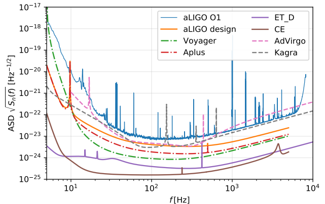
FIG. 1. Evolution of sensitivity of GW interferometric detectors. Text data files for the PSDs or ASDs can be found in [43, 44] under the names given in this table.
