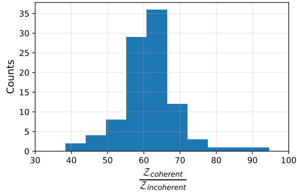
FIG. 10. Histogram of the Bayes factors, for all residuals (except the event highlighted in red in Fig 8 and Table VI), between a coherent (assuming the same incoming signal in all participating detectors) and an incoherent (where the signal in each detector is assumed independent) model [111]. Both the coherent and incoherent models are constructed from a superposition of Morlet-Gabor wavelets, where the number of wavelets is in itself a variable, as implemented in BAYESWAVE [110]. This shows unequivocally that although the modelled analysis, where a known GR waveform approximants attempts to match the signal that best matches what is observed across the detector network, there is a significant fraction of observable coherent signal left. The properties of this left-over signal are not strongly constrained by this analysis however, as expected by the typical SNR \sim 12 for these residual signals. The excluded event, with properties listed in Table VI, has a Bayes factor of \sim 4 \times 10^{11} .
