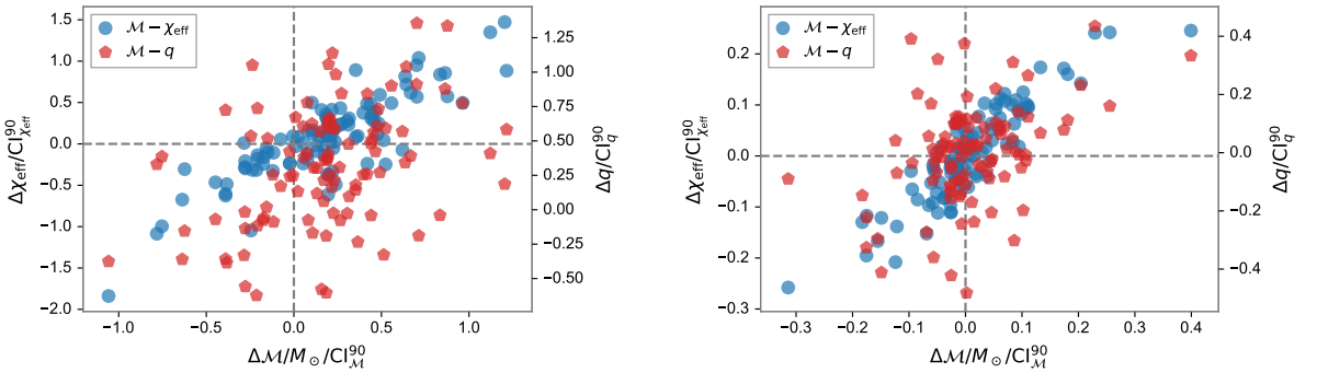
FIG. 6. Ratio of absolute biases and 90% credible intervals \mathcal{R}(\theta, d) as defined in Eq. (11) between chirp-mass \mathcal{M}/M_\odot and effective aligned-spin \chi_{\text{eff}} and chirp-mass and mass-ratio q . \mathcal{R} = \pm 1/2 when the true value is found at the boundaries of the 90% interval. Left: NRSur7dq2 signals recovered with IMRPhenomPv2. Right: IMRPhenomPv2 signals recovered with IMRPhenomPv2.
