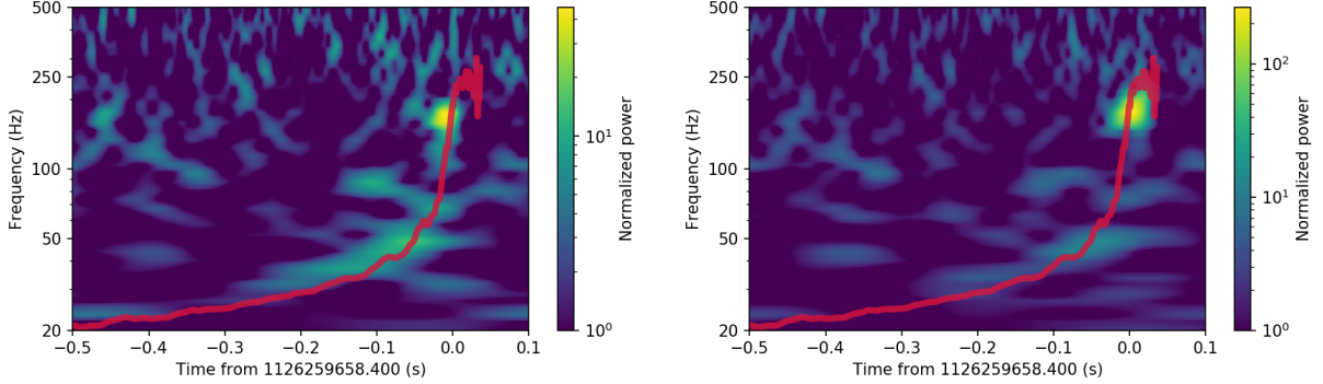
FIG. 9. Q-transform of strain residuals for the event with the loudest residual (optimal network SNR 18.372). The parameters for this event are given in Table VI. The strain residuals were computed by subtracting the IMRPhenomPv2 MAP template from the NRSur7dq2 signal for each detector. Gaussian colored noise was added to the residual before computing the Q-transform. Left : Residual in the interferometer where the residual is loudest: LIGO Hanford, SNR 11.5. Right : Coherent sum of the time-shifted residuals in LIGO Hanford, LIGO Livingston, Virgo and KAGRA. The normalized power is shown in color. The chirp-trace of the injected NRSur7dq2 signal is shown in crimson.
