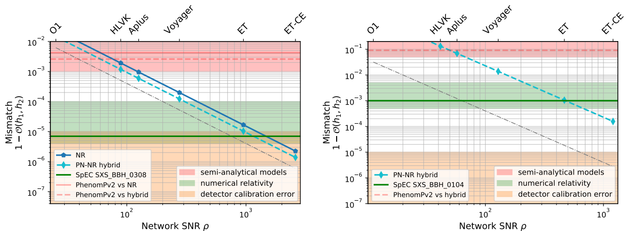
FIG. 2. Predicted waveform accuracy requirements for second and third generation ground based detector networks. We show results for two binaries left : SXS_BBH_0308, and right : SXS_BBH_0104 (see Table I). Each panel shows mismatch against network SNR and on the top x-axis the detector network (see Table II) in which the signal had the SNR shown in the bottom x-axis. Solid lines indicate results for pure NR signals, while dashed lines come from NR signals hybridized against PN waveforms in the inspiral. The blue lines and data points show how the mismatch falls with rising SNR according to the indistinguishability criterion Eq. (8) with the prefactor D tuned according to Eq. (9), as D/(2\rho^2) . The dash-dotted gray line shows the prediction of Eq. (8) with D = 8 . Horizontal red lines show the mismatch of the signal against the IMRPhenomPv2 template waveform at the signal parameters (also called “unfaithfulness”) for aLIGO design sensitivity. The horizontal green line shows the mismatch between NR waveforms obtained for different grid resolutions for the same signal configuration. Shaded regions provide rough estimates of the accuracy of current semi-analytic waveform models and current NR waveforms for the particular binary systems and the level of expected detector calibration error in terms of mismatch. Waveform error estimates are higher for the more challenging unequal mass spinning SXS_BBH_0104 configuration compared to SXS_BBH_0308.
