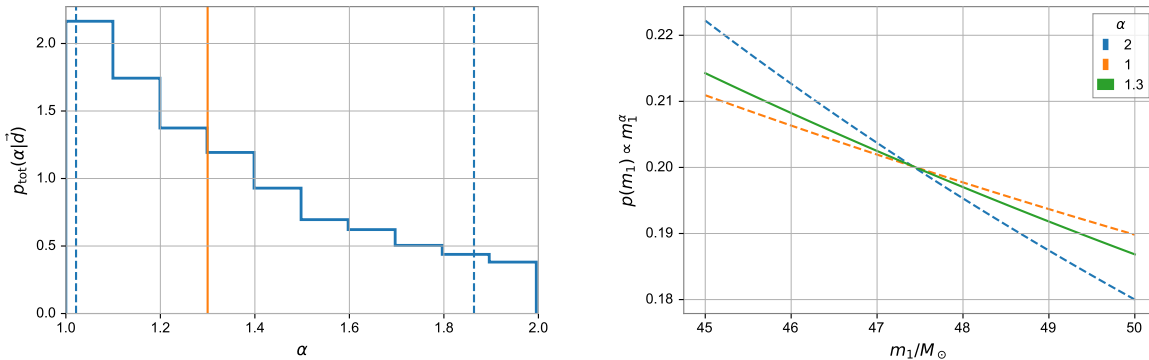
FIG. 11. Left: hyper-posterior p_{\text{tot}}(\alpha|\vec{d}) for power-law index \alpha for m_1 . Right: power-law PDFs for m_1 for \alpha = 1.3 (true value), and the bounds of the uniform hyper-prior on \alpha : \alpha = 1, 2 .
