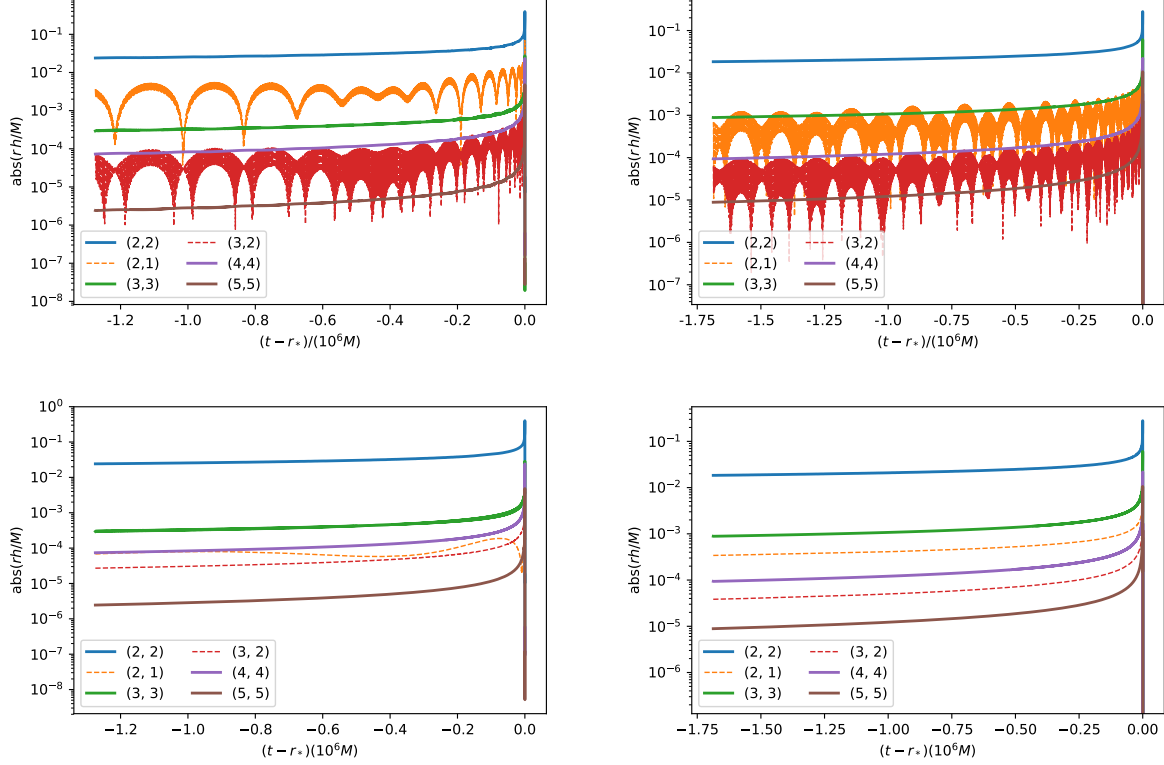
FIG. 14. Selected modes for PN-NR hybrids with the SpinTaylorT1 approximant. Waveform modes are shown in the inertial frame (top panel) and co-precessing frame (bottom panel). The hybrids start at an orbital frequency of M\Omega = 0.002 . Left : SXS_BBH_0308 Right : SXS_BBH_0104 Modes in the co-precessing frame are close to non-precessing waveforms, while inertial modes are modulated by the precession of the orbital plane.
