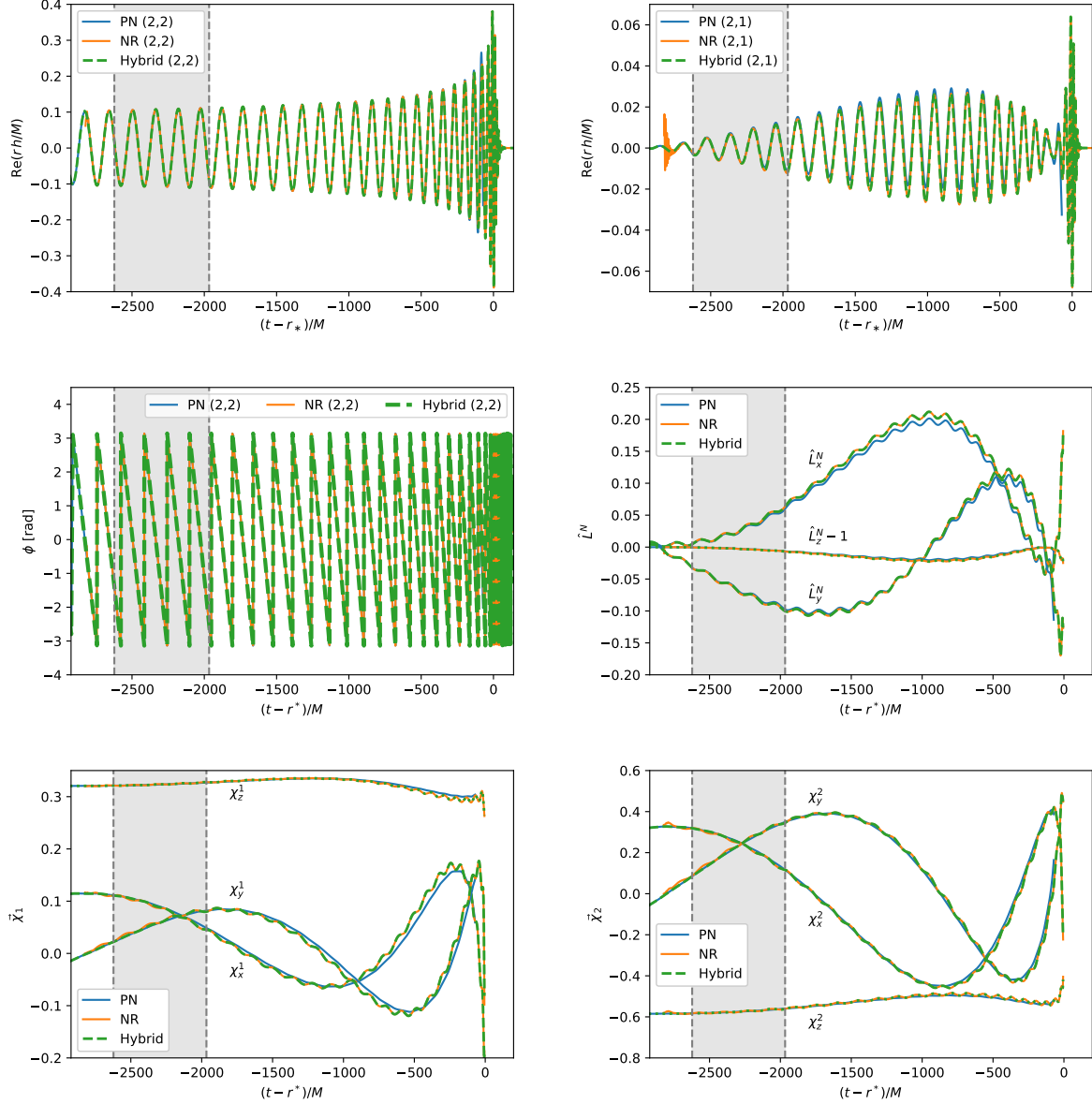
FIG. 12. PN-NR hybrid for SXS_BBH_0308 with the SpinTaylorT1 approximant. For each quantity we show the PN, NR and hybrid data as a function of retarded time before merger. The waveforms have been blended together in the gray shaded hybridization region. Top : real part of the (2,2) and (2,1) modes in the inertial frame Middle: left : (wrapped) phase of the (2,2) mode in the inertial frame right : Cartesian components of the Newtonian orbital angular momentum unit vector in the inertial frame Bottom : Dimensionless spin vectors of the BHs.
