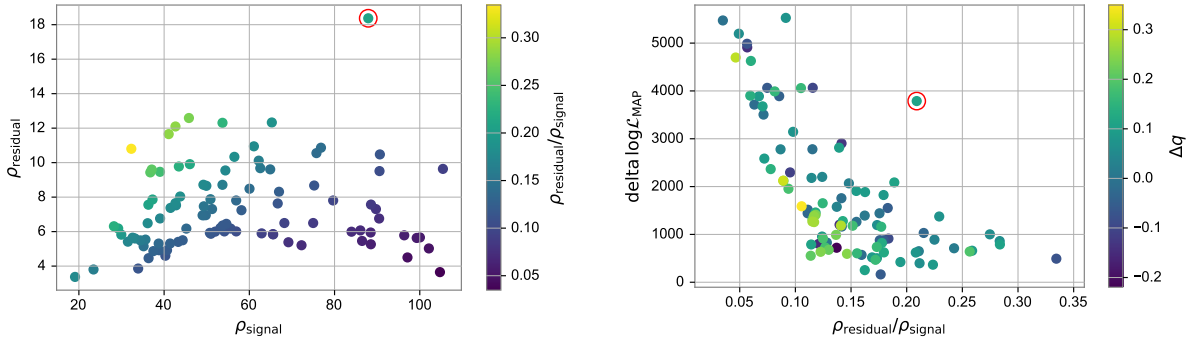
FIG. 8. Fractional network SNR in strain residuals h_s(t; \theta_s) - h_m(t; \theta_{\text{MAP}}) between the NRSur7dq2 signal strains h_s(t; \theta_s) and IMRPhenomPv2 MAP template strain h_m(t; \theta_{\text{MAP}}) for each detector in the HLVK network compared to the SNR of the respective signal strain. Left : Residual SNR as a function of signal (injection) SNR with fractional SNR indicated by color for the events in the population study. Right : Delta Log-likelihood \langle d|h \rangle - 0.5\langle h|h \rangle at MAP against fractional SNR colored by the mass-ratio bias. The bias in mass-ratio is indicated by color. The event with the highest residual SNR is indicated by a red circle around the marker. The parameters for this event are given in Table VI.
