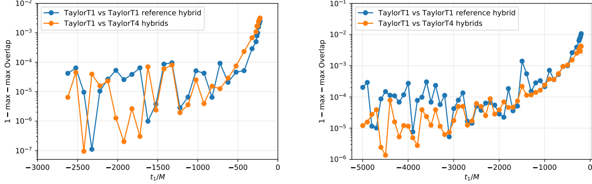
FIG. 15. Mismatch between PN-NR hybrid waveforms. Left : SXS_BBH_0308. Right : SXS_BBH_0104. The mismatch is computed as one minus the max – max overlap including higher modes up to \ell = 8 in the NR waveforms. Here, hybrids are constructed from an orbital frequency of M\Omega = 0.01 and the overlap integral starts at 10 Hz and uses the aLIGO design PSD. (Therefore, higher harmonics will be incomplete in the frequency band, but in a consistent manner. Degradation of the mismatch will come from high frequencies close to merger.) The blue curves show mismatches between SpinTaylorT1 -NR hybrids constructed with a 100M hybridization window as a function of the start time t_1 of this window before merger against a reference hybrid with a broader window at t = [200, 800]M measured from the beginning of the NR waveform, and after the relaxation time. The binaries merge at 2822.24M and 5196.2M from the beginning of the NR simulations, respectively for SXS_BBH_0308 and SXS_BBH_0104. The orange curves show mismatches between SpinTaylorT1 -NR and SpinTaylorT4 -NR hybrids constructed with the same 100M hybridization window as a function of the start time t_1 .
