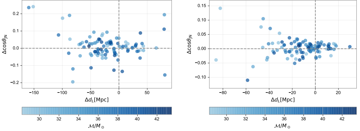
FIG. 7. Absolute biases \theta_s - \theta_{\text{MAP}} between luminosity distance and the cosine of the inclination angle Left: NRSur7dq2 signals recovered with IMRPhenomPv2. Right: IMRPhenomPv2 signals recovered with IMRPhenomPv2. As in Fig. 5 we indicate the signal chirp mass by the luminosity of the symbol colors.
