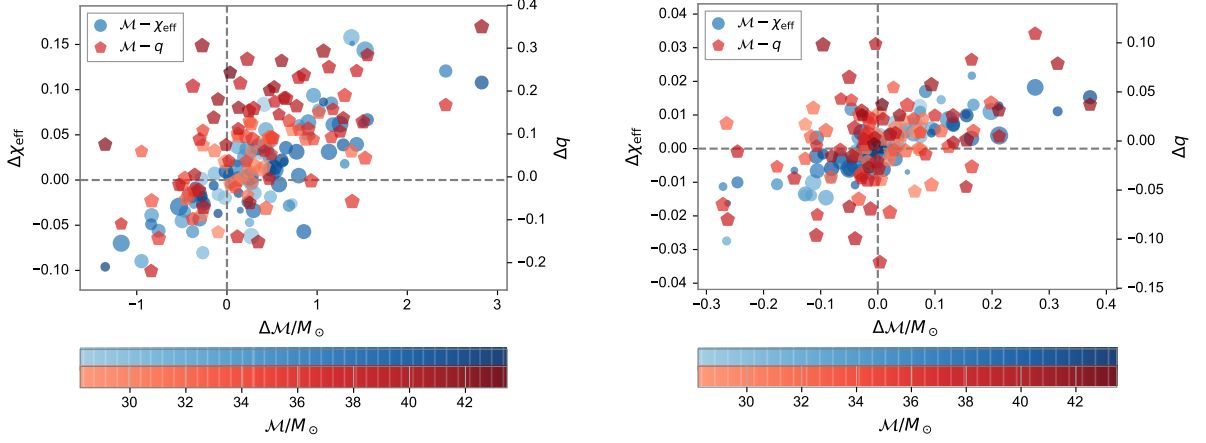
FIG. 5. Absolute biases \theta_s - \theta_{\text{MAP}} between chirp-mass \mathcal{M}/M_\odot and effective aligned-spin \chi_{\text{eff}} (blue circles) and chirp-mass and mass-ratio q (red pentagons). Left: NRSur7dq2 signals recovered with IMRPhenomPv2. The Pearson correlation coefficients are R_{\mathcal{M},\chi_{\text{eff}}} \sim 0.8 and R_{\mathcal{M},q} \sim 0.5 . Right: IMRPhenomPv2 signals recovered with IMRPhenomPv2. The Pearson correlation coefficients are R_{\mathcal{M},\chi_{\text{eff}}} \sim 0.8 and R_{\mathcal{M},q} \sim 0.3 . We indicate the signal chirp mass by the luminosity of the symbol colors and the absolute value of the effective aligned-spin and mass-ratio of the signal by the symbol area to give a sense of how the biases are distributed over the parameter space. The symbol area was calculated as 200\sqrt{|\chi_{\text{eff}}|} and 100\sqrt{q} .
