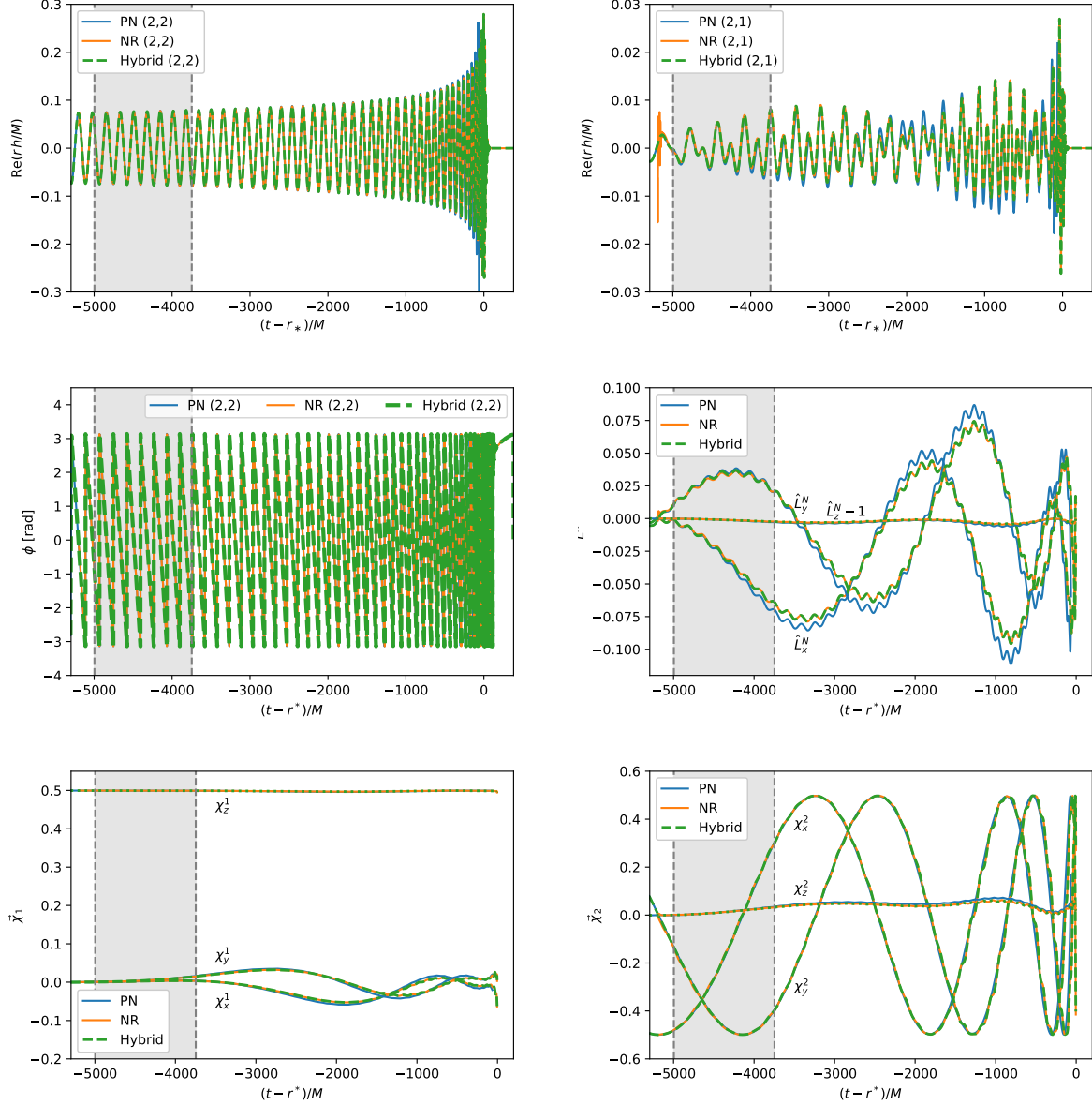
FIG. 13. PN-NR hybrid for SXS_BBH_0104 with the SpinTaylorT1 approximant. For each quantity we show the PN, NR and hybrid data as a function of retarded time before merger. The waveforms have been blended together in the gray shaded hybridization region. Top : real part of the (2,2) and (2,1) modes in the inertial frame Middle: left : (wrapped) phase of the (2,2) mode in the inertial frame right : Cartesian components of the Newtonian orbital angular momentum unit vector in the inertial frame Bottom : Dimensionless spin vectors of the BHs.
