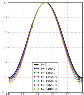
Figure 2: Radial structure of the electrostatic potential \phi at different simulation times for a GYSELA simulation with parameters given in Table 2. k_r \rho_i \simeq 0.039 is almost preserved between initial time (black line) and final time t = 24800\Omega_{c0} .
