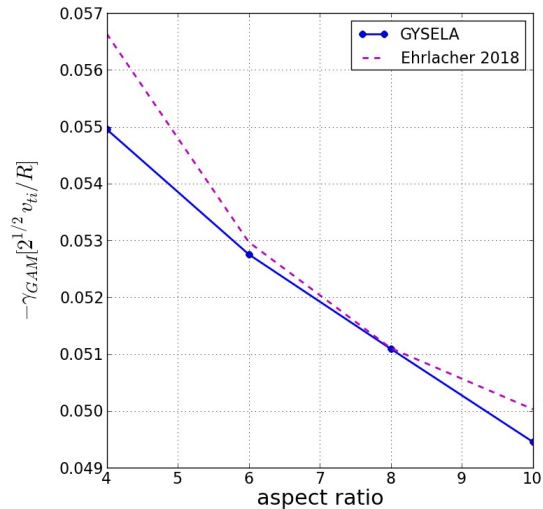
Figure 10: Damping rate of the radial electric field versus aspect ratio measured with GYSELA code (blue line). The dotted magenta line on the left graph corresponds to the analytical expression of \gamma given by Eq.(18).
