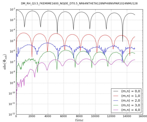
Figure 3: Time evolution of the five Fourier modes of the electrostatic potential \tilde{\phi}_{m0}(r = 0.5a, t) with m = \{0, 1, 2, 3, 4\} for a simulation which parameters are described in Table 2.
