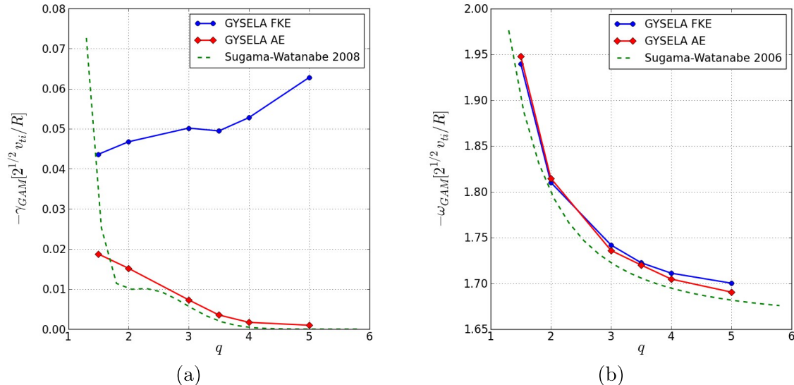
Figure 8: Damping rate (a) and frequency (b) of the radial electric field versus the safety factor q measured with GYSELA code for two types of simulations: adiabatic electrons (GYSELA AE-red line) and kinetic electrons (GYSELA FKE-blue line). The dotted green lines correspond to the explicit formulas of the damping rate and the frequency given by Sugama and Watanabe in [25] (see Eq. (19)).
