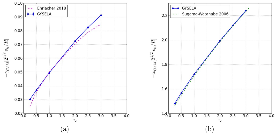
Figure 7: Damping rate (a) and frequency amplitude (b) of the radial electric field versus \tau_e measured with GYSELA code (blue line). The dotted magenta line in (a) corresponds to the analytical expression of \gamma given by Eq.(18) while the dotted green line in (b) is the analytical prediction given by Sugama & Watanabe in [25].
