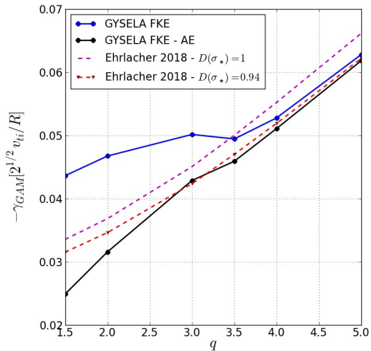
Figure 9: Damping rate of the radial electric field versus the safety factor q measured with GYSELA code (blue line). The dotted lines correspond to the analytical expression of \gamma given by Eq.(10): with \mathcal{D}(\sigma^*) = 1 (magenta line) and with \mathcal{D}(\sigma^*) = 0.94 (red line).
