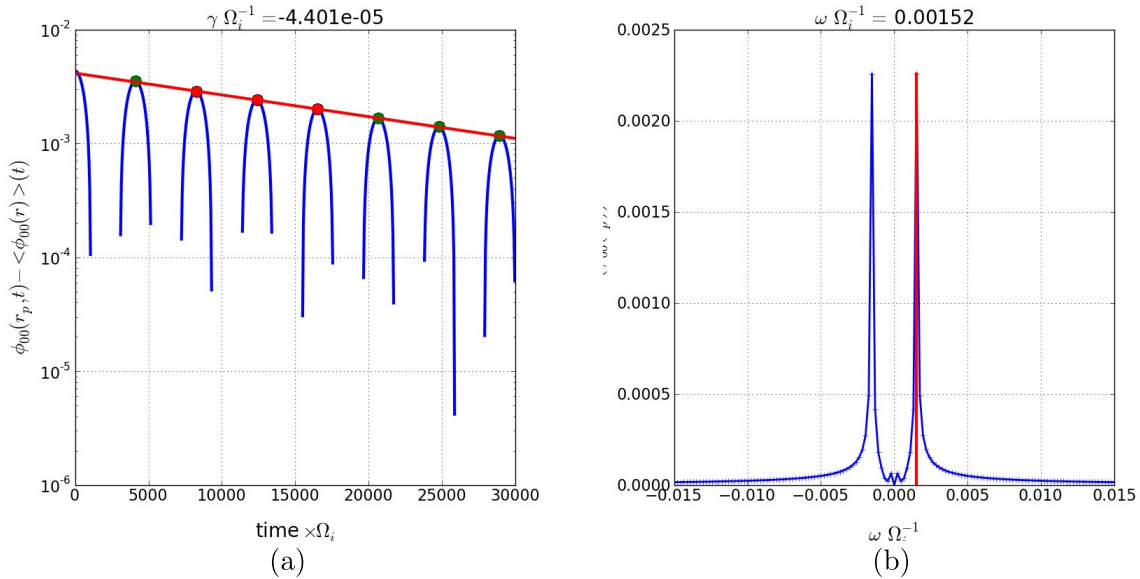
Figure 4: Simulation results for numerical parameters given in Table 2: (a) Time evolution of \log(\phi(r_p, t) - \langle \phi_{00} \rangle_r(t)) ( r_p = 0.5a ) with an approximate value of the damping rate \gamma \Omega_{c_0}^{-1} \simeq 4.4 \cdot 10^{-5} given by the slope of the red line ; (b) Fourier transform in time of \phi(r_p, t) which gives an approximation of the GAM frequency equal to \omega \Omega_{c_0}^{-1} \simeq 0.0015 .
