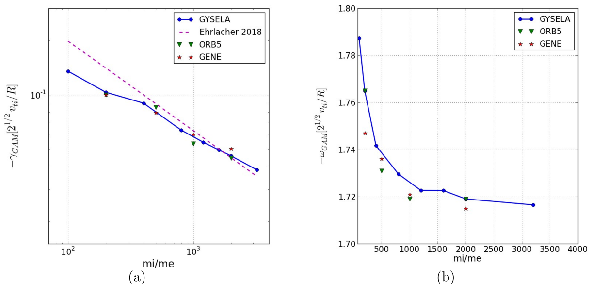
Figure 5: Damping rate (a) and frequency amplitude (b) of the radial electric field versus m_i/m_e measured with GYSELA code (blue line) and compared to ORB5 (green triangles) and GENE (red stars) codes published in [1]. The dotted magenta line in (a) corresponds to the analytical expression of \gamma given by Eq.(18).
