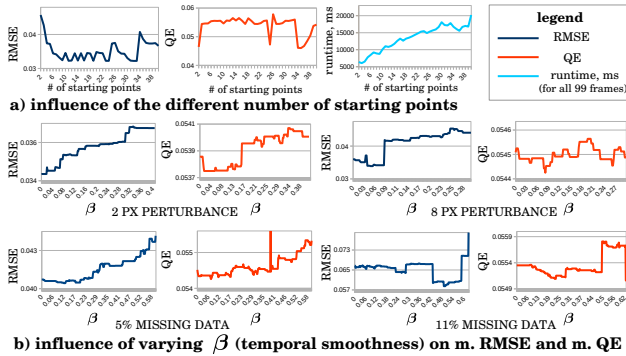
Figure 3: Results of the experiments with SGD parameters: (a) the influence of the different number of starting points is evaluated on the measurements without noise; (b) the influence of \beta is evaluated on perturbed tracks and tracks with missing data with 20 starting points. In both cases, the shapes of seq. B are taken as a DSP and the clean tracks of seq. A are taken as the incoming dense point tracks. Mind the scaling of the y -axis.
