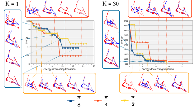
Figure 4: The sequences of energy-decreasing transitions and the corresponding energy values observed in our sampler, for transformation estimation ( K = 1 ) and point set alignment with K = 30 interactions per \mathbf{x}_n . Besides the graphs, we visualise alignment results for selected energy values and the angle of initial misalignment \theta \in \{\frac{\pi}{8}, \frac{\pi}{4}, \frac{\pi}{2}\} .
