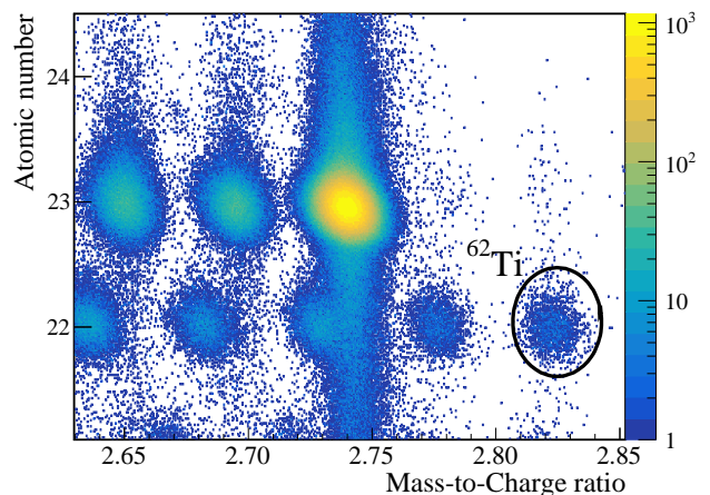
Figure 1: Particle identification plot for the outgoing fragments measured with the SAMURAI dipole magnet and related detectors. Incoming ^{63}\text{V} isotopes were selected with BigRIPS. ^{62}\text{Ti} isotopes are indicated by the ellipse.
