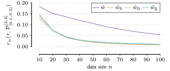
Figure 3: Average regret. Regret r_n(\tau, \mathcal{P}_{[0.1, 0.5]}^{[2, 4]}) for sample sizes n = \{10, \dots, 100\} and estimators \tau = \{\hat{w}, \hat{w}_0, \hat{w}_{\bar{0}}, \bar{w}_{\bar{0}}\} .
