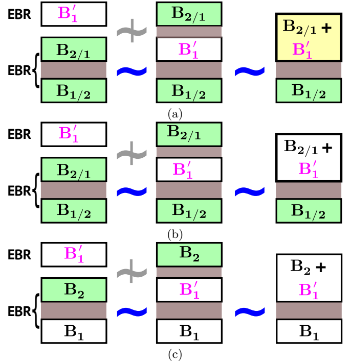
FIG. 10. Fragile topology of the split EBR of the honeycomb lattice B_1 + B_2 , with B_1 = B_1^{a/b}(2b) and B_2 = B_2^{a/b}(2b) , under the coupling with the trivial EBR of the triangular lattice, B_1' = B_1^{a/b}(1a) . Two-band (four-band) subspaces with non-zero Wilson loop winding are colored in green (yellow), otherwise in white. In (a) and (b) we choose either B_1 or B_2 as the two-band occupied subspace of the six-band insulating phases, in (c) it can only be B_1 . The band gaps are drawn in brown. The blue \sim marks that the coupling is adiabatic, i.e. without closing the band gap, while the barred gray marks a non-adiabatic coupling (i.e. closing the band gap). (a) reveals a stable topology of the split EBR (i.e. here for a nonzero Fu-Kane-Mele invariant). (b) and (c) reveal a fragile topology of the split EBR (i.e. nonzero two-band Wilson loop winding but with a zero Fu-Kane-Mele invariant). (c) corresponds to the example given in Ref. 51, and here in Fig. 9.
