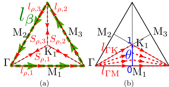
FIG. 5. (a) Symmetry decomposition of the HBZ patch S_\beta = S_{\rho,1} + S_{\rho,2} + S_{\rho,3} bounded by l_\beta \sim l_{\rho,3} \circ l_{\rho,2} \circ l_{\rho,1} . (b) Loop parametrization of the patch S_\rho = \bigcup_{\theta \in [0,1]} l_\theta with l_0 = l_{\Gamma\text{M}} and l_1 = l_{\Gamma\text{K}} .
