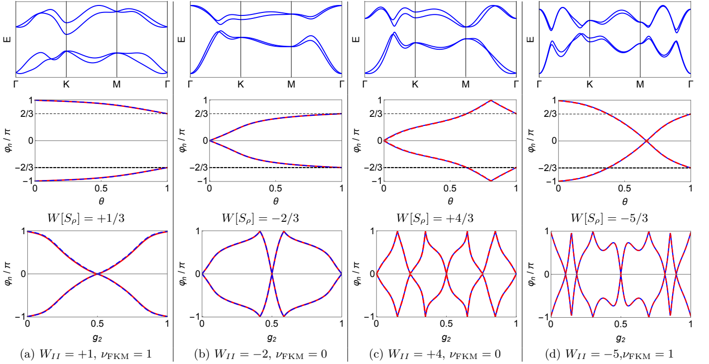
FIG. 6. Spinful topological phases obtained for SOC that breaks inversion symmetry only adiabatically. Columns (a-d) correspond to those of Fig. 3. First row: band structures along the high symmetry lines of the BZ. Second row: spectral flow of the Wilson loop over one patch S_\rho parameterized by loop sections l_\theta from l_{\Gamma M} ( \theta = 0 ) to l_{\Gamma K} ( \theta = 1 ). Third row: spectral flow of the Wilson loop over the whole BZ parameterized by loop sections \{l_{g_2}\}_{g_2 \in [0,1]} with l_{g_2=0.1} = l_{\Gamma M} and l_{g_2=0.5} = l_{MM} . Blue (red) dashed lines give the Wilson loop of the two-band occupied (unoccupied) subspace. For each case the Wilson loop winding over a sixth BZ patch W[S_\rho] (computed with respect to reference Wilsonian phase marked by a thick black line), the Wilson loop winding W_{II} , and the Fu-Kane-Mele \mathbb{Z}_2 invariant is given. Importantly, the agreement between the second and the third rows confirms that the total winding of the Wilson loop over the BZ (protected by C_2\mathcal{T} symmetry) does not depend on the parameterization of the flow.
