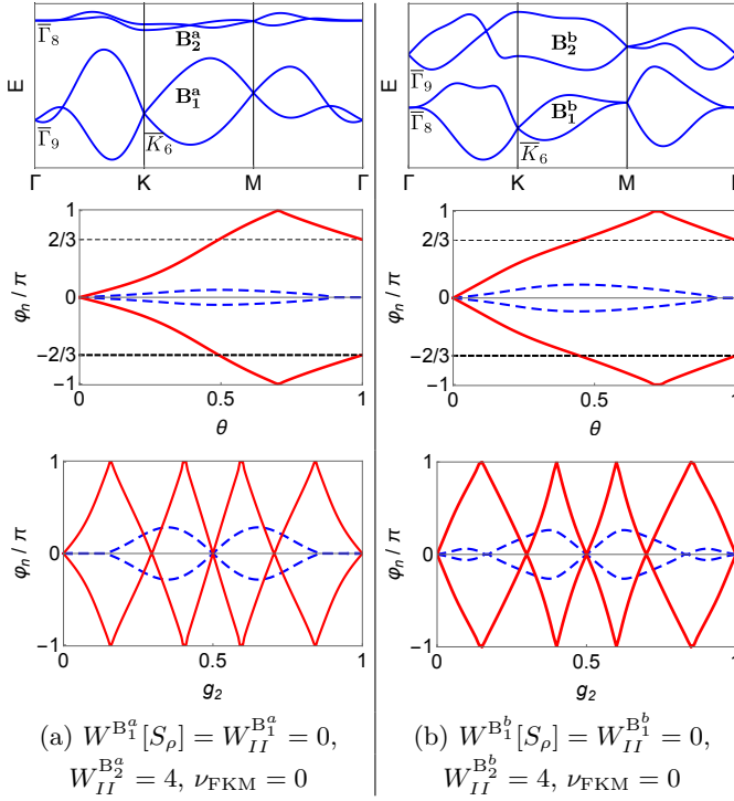
FIG. 7. Spinful topological phases with Rashba SOC breaking inversion symmetry non-adiabatically. First, second and third rows are similar to Fig. 6. (a) EBR split as B_1^a + B_2^a with B_1^a = (\bar{\Gamma}_9, \bar{K}_6, \bar{M}_5) and B_2^a = (\bar{\Gamma}_8, \bar{K}_4, \bar{K}_5, \bar{M}_5) , with the parameters chosen as in Ref. 51 for comparison. (b) EBR split as B_1^b + B_2^b with B_i^b = B_i^a[\bar{\Gamma}_9 \leftrightarrow \bar{\Gamma}_8] .
