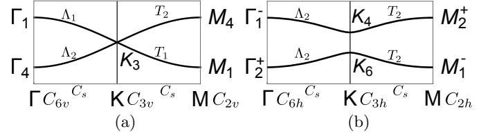
FIG. 2. Examples of band structures for the EBRs of (a) spinless symmetry class A+L77(2b) \cong AI+L80(2b) , and (b) spinless symmetry class A+L75(2b) , when restricted to Wyckoff’s position 2b. Notations from the Bilbao Crystallographic Server 58 for the IRREPs of the space groups.
