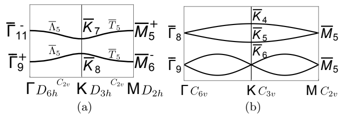
FIG. 4. EBRs for (a) spinful symmetry class AII+L80(2b), and (b) spinful symmetry class AII+L77(2b), when restricted to the Wyckoff's position 2b. Notations from the Bilbao Crystallographic Server 58 for the IRREPs of the space groups.
