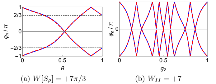
FIG. 11. Example of a split EBR with a Wilson loop winding of W_{II} = +7 . (a) Flow of the Wilsonian phases over the patch S_\rho . (b) Flow of the Wilsonian phases over the BZ.
