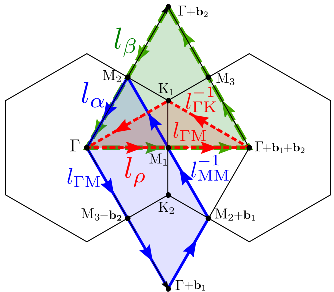
FIG. 1. First BZ of the honeycomb lattice spanned by the primitive reciprocal vectors \mathbf{b}_1 and \mathbf{b}_2 . High-symmetry points (HSP) \Gamma , K and M. Inequivalent high-symmetry points are written with different subscripts, i.e. K_1 , K_2 , M_1 , M_2 , M_3 . Half Brillouin zone (HBZ) patches S_\alpha (blue) and S_\beta (green), with their respective oriented boundaries l_\alpha \sim l_{MM}^{-1} \circ l_{\Gamma M} (blue) and l_\beta (dashed green), and the patch S_\rho (red) bounded by l_\rho = l_{\Gamma K}^{-1} \circ l_{\Gamma M} (dotted red) covering one sixth of the BZ. l_{P_2 P_1} is the oriented open loop that threads the BZ starting at point P_1 , crossing P_2 and ending at the shifted point P_1 + \mathbf{K} with the reciprocal lattice vector \mathbf{K} = \pm \mathbf{b}_{1(2)} . We mean by \sim equal up to segments that cancel each other through a translation by a reciprocal lattice vector. Note that the different segments of the curves directly correspond to the underlying crystal symmetries.
