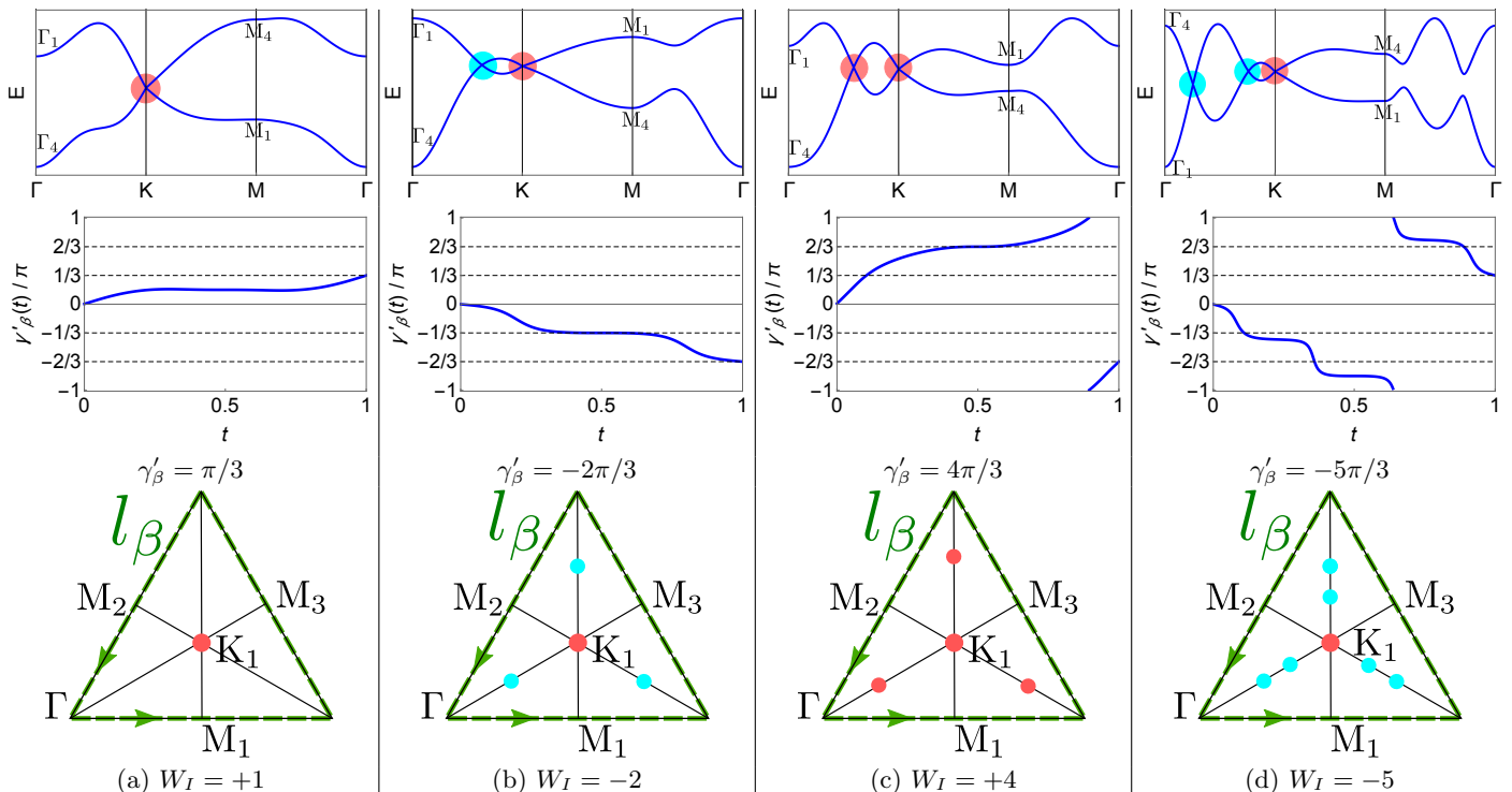
FIG. 3. Spinless topological semi-metallic phases of the honeycomb lattice reached through band inversions at \Gamma and M triggered by tight-binding parameters of increasing range. Columns (a-d) correspond to an increasing number of simple nodal points protected by crystalline symmetries. First row: band structures along the high symmetry lines of the BZ. Second row: noncyclic Berry phase along one third of the C_3 -symmetric loop l_\beta encircling K . Third row: schematic configuration of symmetry protected nodal points within the HBZ S_\beta bounded by l_\beta (nodal points in red have W_I = +1 , and in blue W_I = -1 ). Crystalline winding numbers are (a) W_I = \gamma_\beta/\pi = +1 , (b) W_I = -2 , (c) W_I = +4 , and (d) W_I = -5 .
