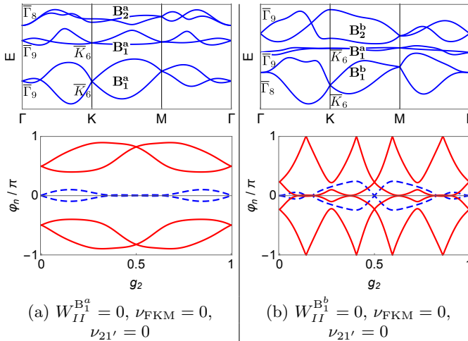
FIG. 9. Similar to Fig. 8, but here the six-band topological phases are obtained from the four-band phases of Fig. 7 where inversion symmetry is broken non-adiabatically through Rashba SOC. (a) Split EBR B_1^a + B_2^a , corresponding to the case discussed in Ref. 51. (b) Split EBR B_1^b + B_2^b .
