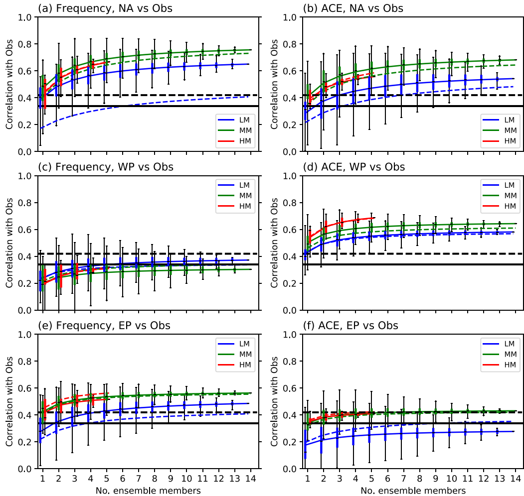
FIG. 10. Correlation of (left) model tropical cyclone frequency and (right) ACE 925 for the (a),(b) North Atlantic (NA), (c),(d) northwestern Pacific (WP), and (e),(f) northeastern Pacific (EP) over 1979–2014 against observations for ensembles of HadGEM3-GC31 simulations [a total of 14 members at both MM (100 km) and LM (250 km) resolution, and 5 members at HM (50 km) resolution]. For each combination of n ensemble members ( x axis), a box and whiskers are plotted (the box shows the lower–upper quartile range, with a line at the median, and the whiskers show the range of the data). The mean correlations for each n ensemble member correlation are joined up by the line. The solid lines are for TRACK, and the dashed lines are for TempestExtremes. The solid and dashed black lines are approximations of the 95% and 99% confidence levels, respectively (assuming that each of the 36 years is an independent sample).
