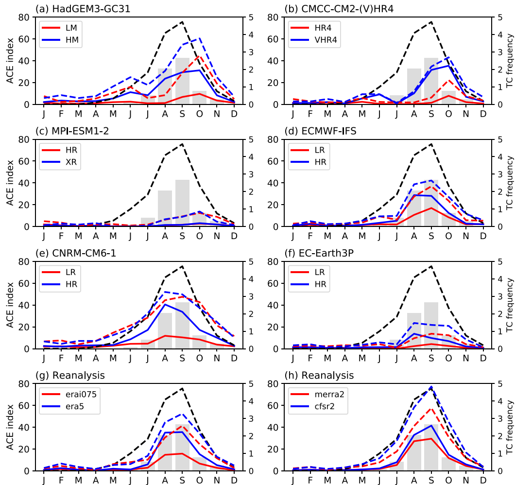
FIG. 9. Mean seasonal cycle of tropical cyclone ACE and frequency in the North Atlantic for models and re-analyses (using TRACK) and observations. In each plot, the gray bars represent the observed monthly mean ACE over the 1979–2014 period, with the solid lines representing the modeled ACE_{925} . The dashed lines show the TC frequency for observations (black) and models. The red or blue line is the lower or higher resolution, respectively, for each model or reanalysis.
