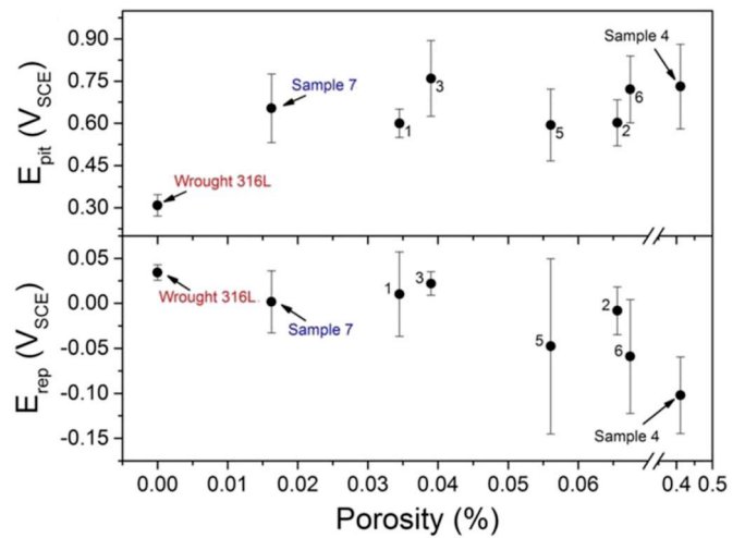
Fig. 9. Pitting and repassivation potentials of L-PBF produced 316L austenitic stainless steel compared to conventionally-produced material. While the resistance to pitting is higher, the repassivation of pits also requires a higher potential. Figure reprinted under Creative Commons license (CC-BY-NC-ND 4.0) from Ref. [55].
