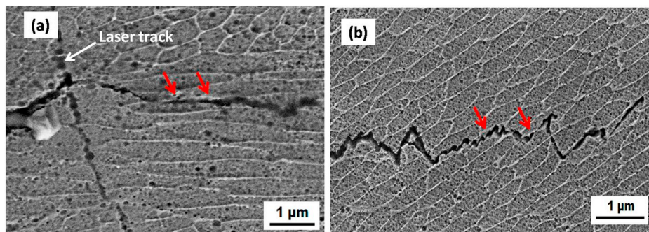
Fig. 8. Cross sectional SEM image (backscattered electron contrast) showing fatigue crack growth interaction with solidification cell structure in loading perpendicular to the grain long axis (a) and parallel to it (b). Note that grains are elongated and coaxial with the solidification cells. Since the crack progresses preferentially along the cell boundaries, the crack tortuosity depends on loading direction. Reproduced with permission from Ref. [26].
