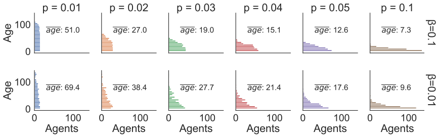
Figure 1. Population pyramids created by removing agents at different turnover rates (columns) using the Gompertz function with two different \beta settings (rows). Increased turnover leads to younger populations, with a lower mean age.
