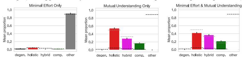
Figure 1. Mean proportions and 95% CIs of language types after convergence (generations 100-150 of 100 simulation runs). Dashed lines show baseline proportions of language types in hypothesis space (black for all types, grey for relative proportions of only the fully expressive language types). P(\text{noise}) = 0.5 , cost ratio OPEN:RESTRICTED = 2:1, transmission bottleneck = 20 data points per learner.
