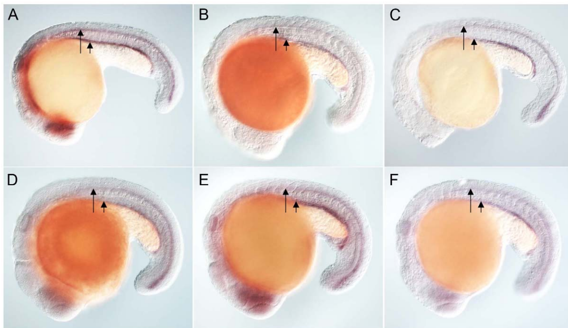
Figure 2. Zebrafish FoxJ2 and FoxJ3 are unable to induce the expression of ciliary genes. (A) Expression of efc1 in the spinal cord (long arrow) and pronephric (kidney) duct (short arrow) of a wild-type zebrafish embryo, and in embryos ectopically expressing zebrafish FoxJ2 (B) and FoxJ3 (C), respectively. (D) Expression of spag6 in the spinal cord (long arrow) and pronephric (kidney) duct (short arrow) of a wild-type zebrafish embryo, and in embryos ectopically expressing zebrafish FoxJ2 (E) and FoxJ3 (F), respectively. Embryos depicted are at 20 hpf, oriented anterior to the left, dorsal to the top.
