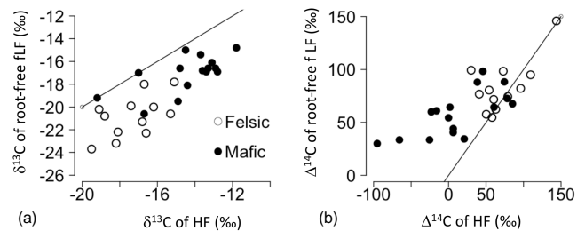
Figure 2. Comparison of ^{13}\text{C} (a) and ^{14}\text{C} (b) in root-free free light fraction (root-free fLF) and heavy fraction (HF) organic C for individual samples from A horizons (see Table 3). Felsic lithologies (white circles) include soils developed on granite and rhyolite; mafic lithologies (black circles) include soils developed on gabbros, basalts, and nephelinite. The 1 : 1 correlation line is plotted for reference.
