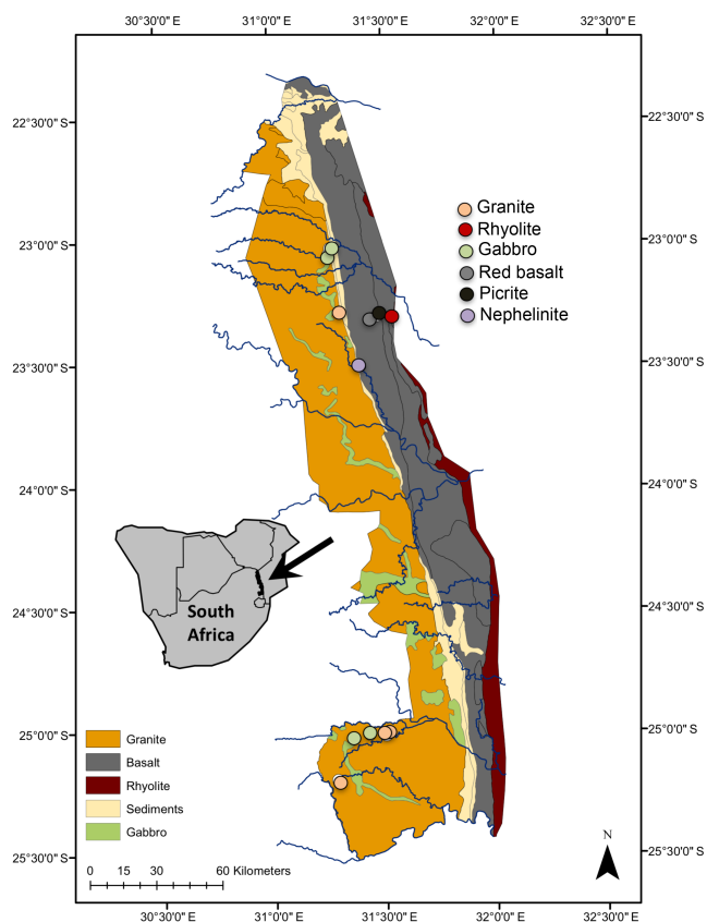
Figure 1. Locations and lithology of parent materials where soils were sampled for this study. Rainfall decreases from \sim 740 \text{ mm a}^{-1} in the southern end of the park to \sim 450 \text{ mm a}^{-1} in the northern end of the park.
