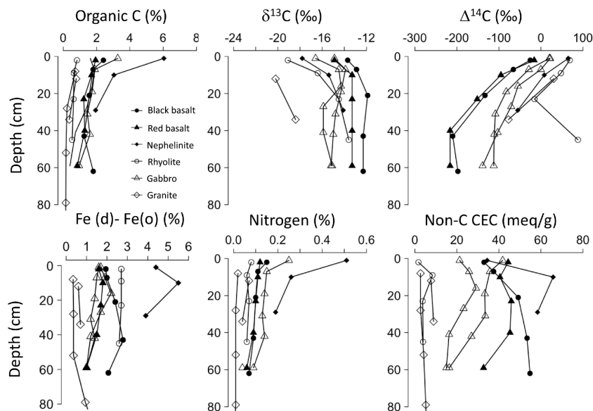
Figure 3. Depth profiles of bulk C (top-left), \delta^{13}\text{C} (top-middle), and \Delta^{14}\text{C} (top-right) measured in bulk C for soil profiles developed on selected lithologies. Also shown in the lower panels are other soil bulk properties, total Fe oxyhydroxides (Fe(d)–Fe(o)) (bottom-left), total nitrogen (bottom middle), and cation exchange capacity (CEC) corrected for organic matter contributions (bottom right; see text).
