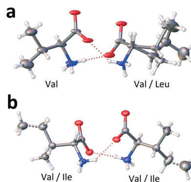
Fig. 11 Occupancy of molecular positions in the dimers of non-equimolar heterocompounds V_3L (a) and V_2I (b). Ellipsoids reflect the 20% and 50% probabilities in the case of V_3L and V_2I , correspondingly. Images are constructed in the service OLEX2. 44
