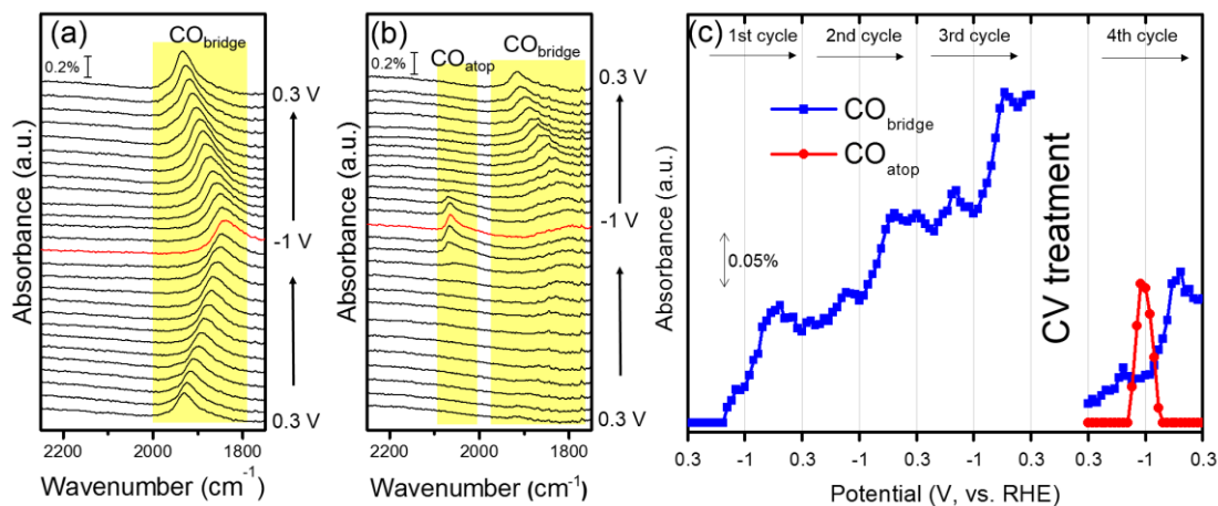
Figure 6. In situ SEIRA spectra of (a) as-prepared Cu electrode obtained in the (a) 3rd cycle and the (b) 4th cycle of CO 2 reduction process (after CV-treated cycles). (c) Potential-dependence of intensity of CO bridge and CO atop -associated peaks during four cycles.
