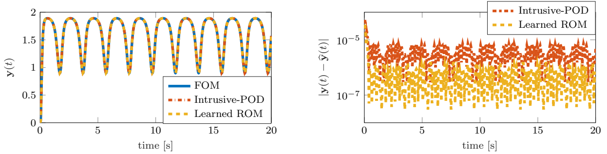
Figure 3: Chafee-Infante example: Output (left) and output errors (right) of the POD intrusive and the learned ROMs of order r = 12 .
