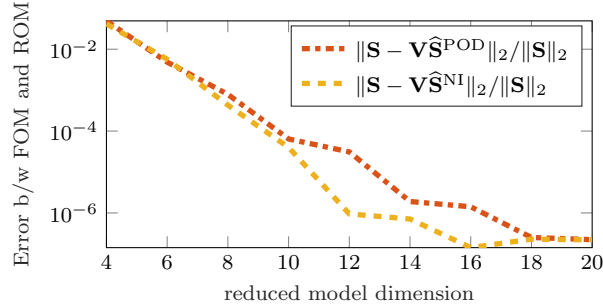
Figure 7: Tubular reactor example: Relative state errors produced by both ROMs, i.e., \|\mathbf{S} - \mathbf{V}\hat{\mathbf{S}}^{\text{POD}}\|_2 / \|\mathbf{S}\|_2 and \|\mathbf{S} - \mathbf{V}\hat{\mathbf{S}}^{\text{NI}}\|_2 / \|\mathbf{S}\|_2 .
