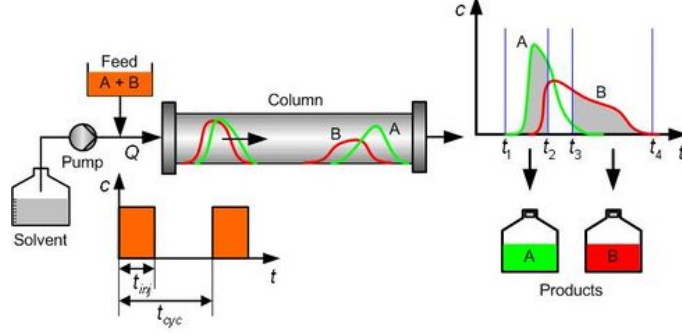
Figure 8: The figure shows a chromatography process, separating a mixture, c.f. [44].
