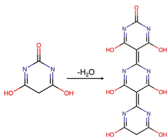
Scheme 1. Idealized illustration of barbituric acid thermal condensation reaction by water elimination forming crystalline trimer.
